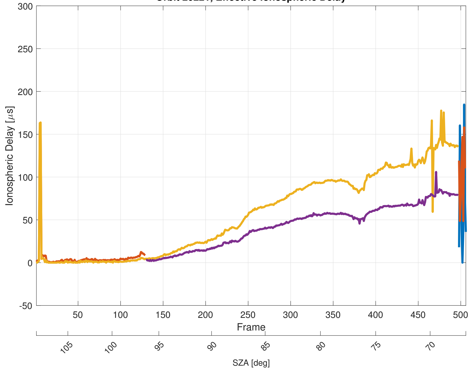
Orbit 20221, Effective Ionospheric Delay
