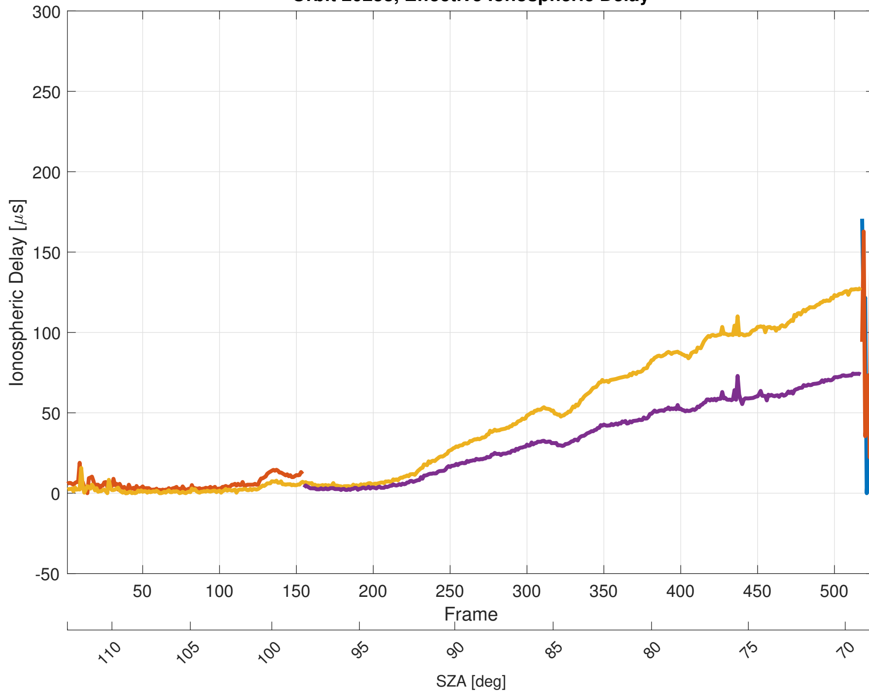
Orbit 20238, Effective Ionospheric Delay
