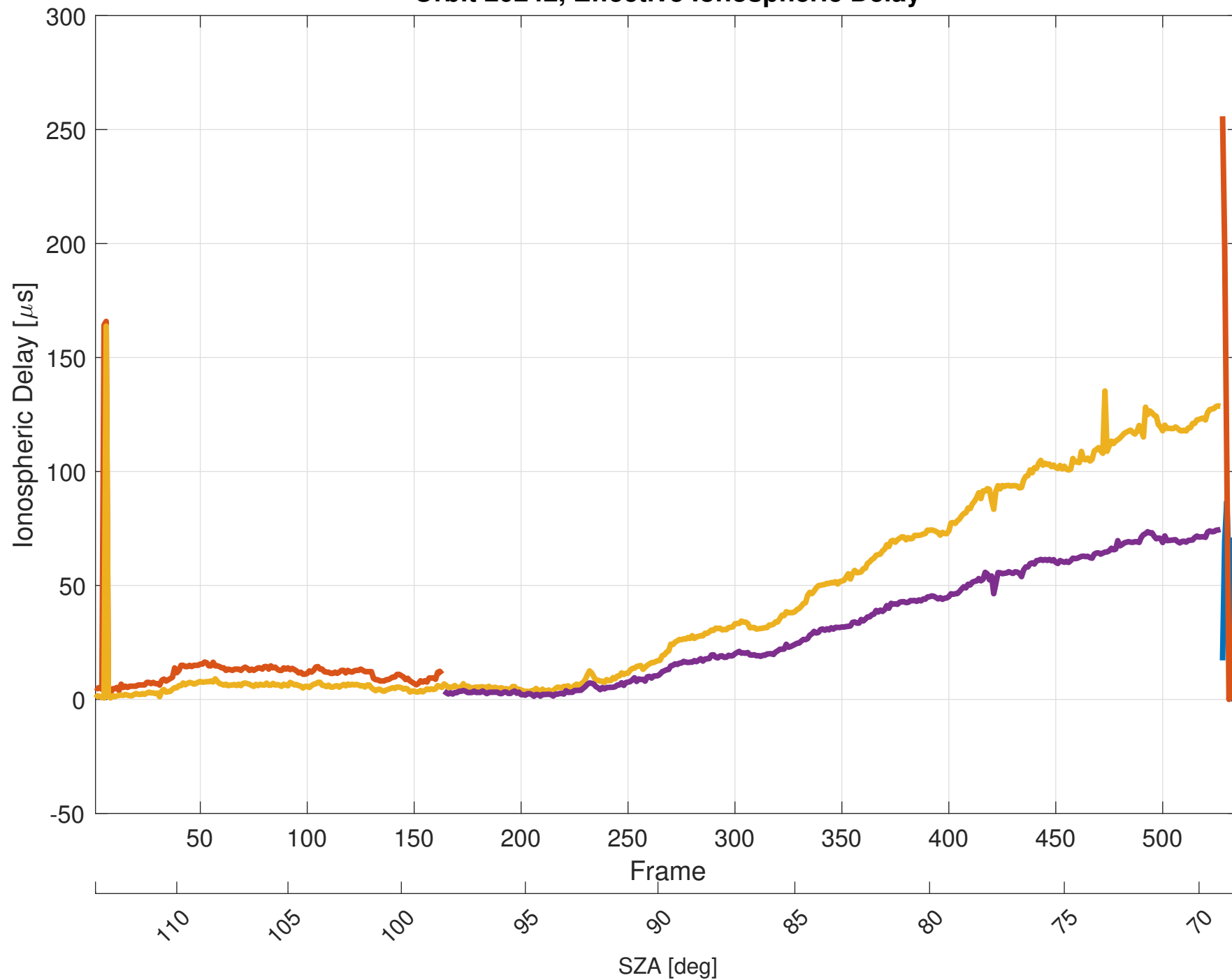
Orbit 20242, Effective Ionospheric Delay
