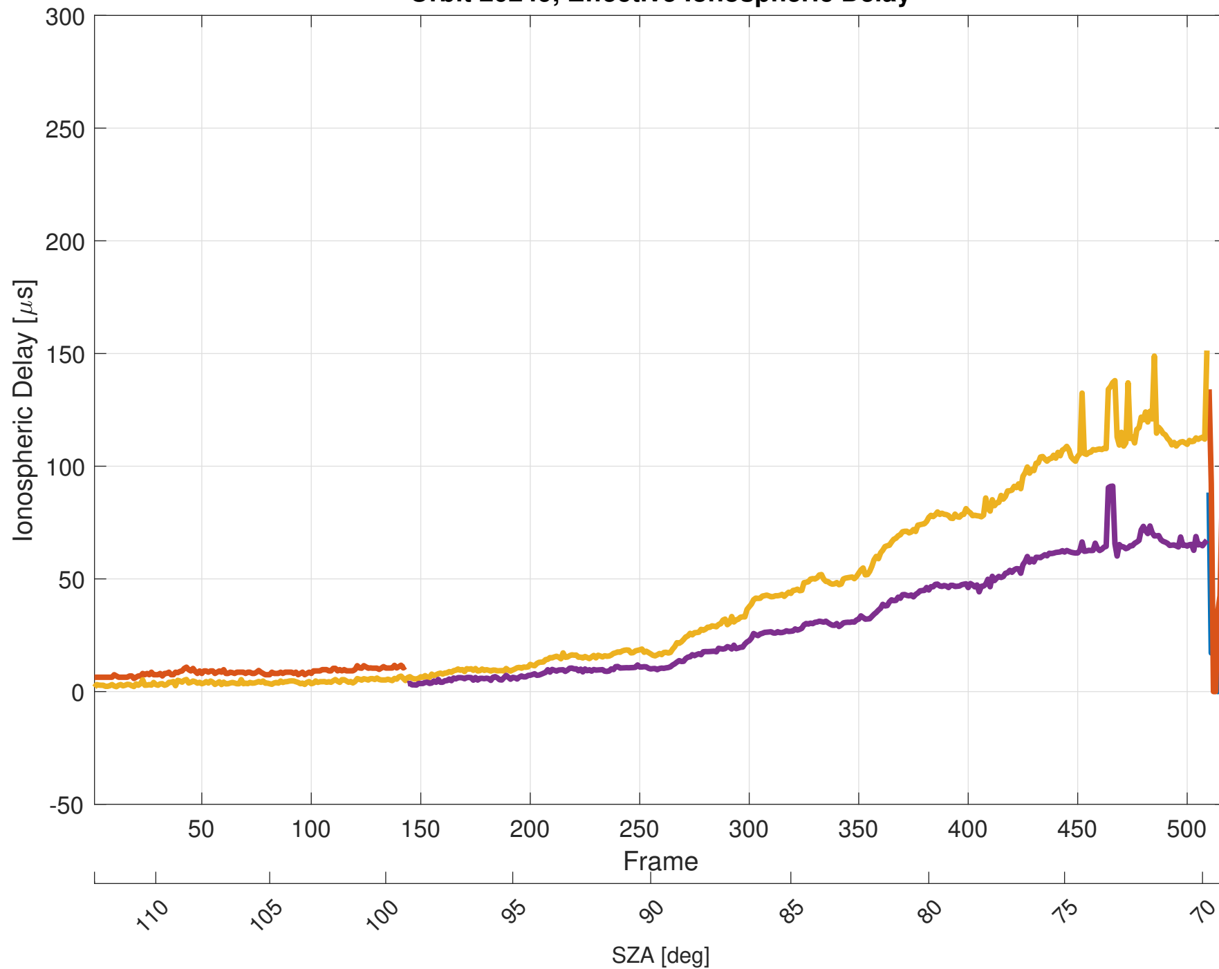
Orbit 20249, Effective Ionospheric Delay
