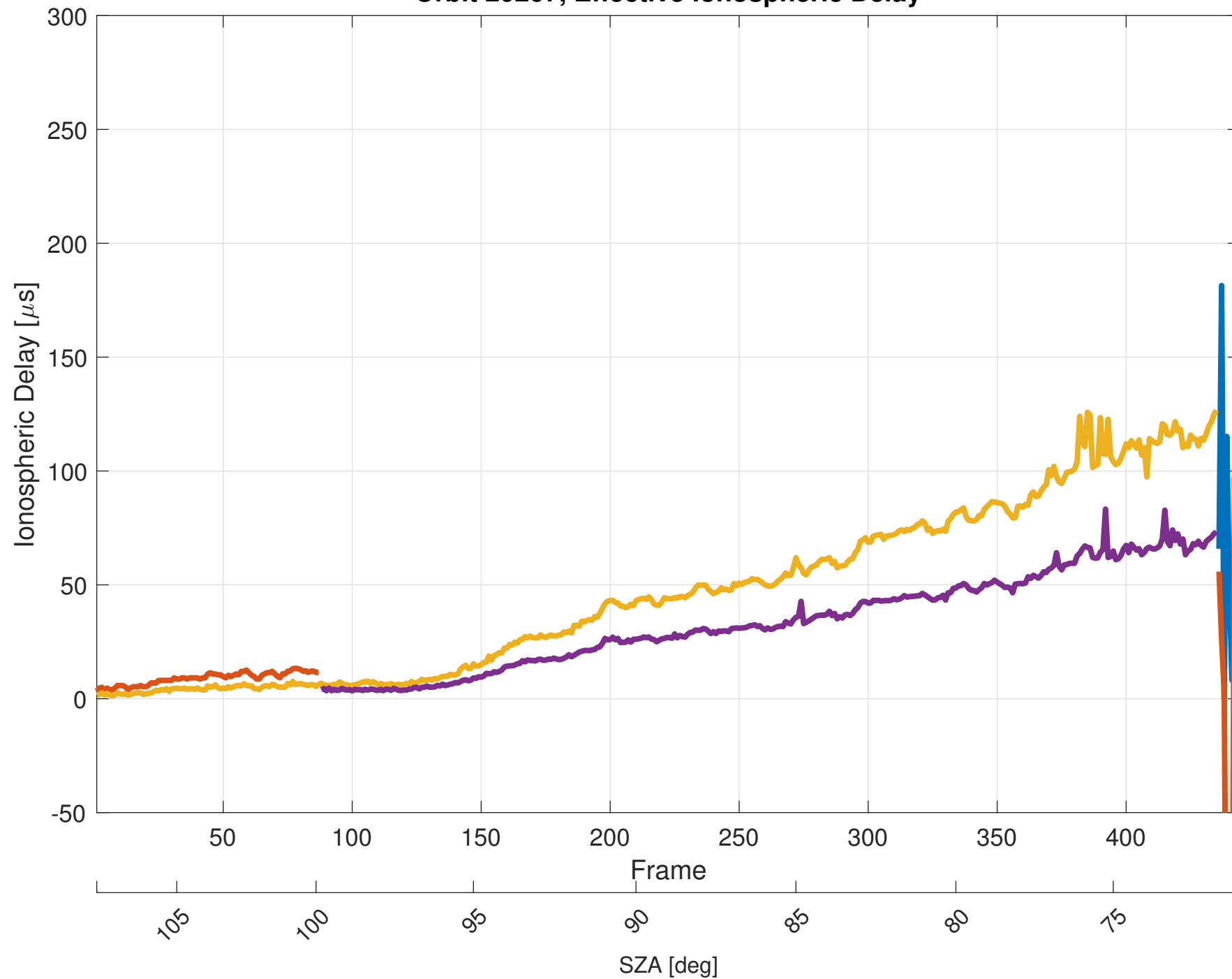
Orbit 20267, Effective Ionospheric Delay
