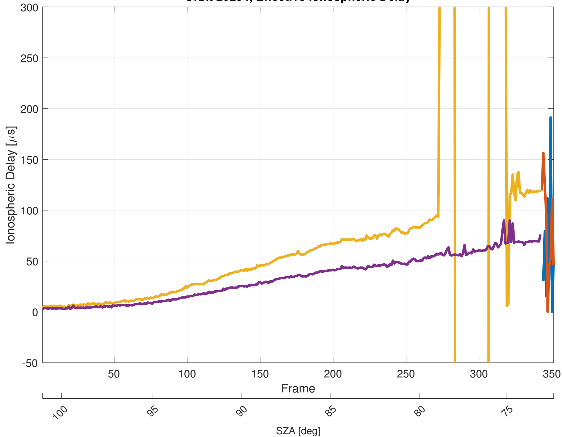
Orbit 20294, Effective Ionospheric Delay
