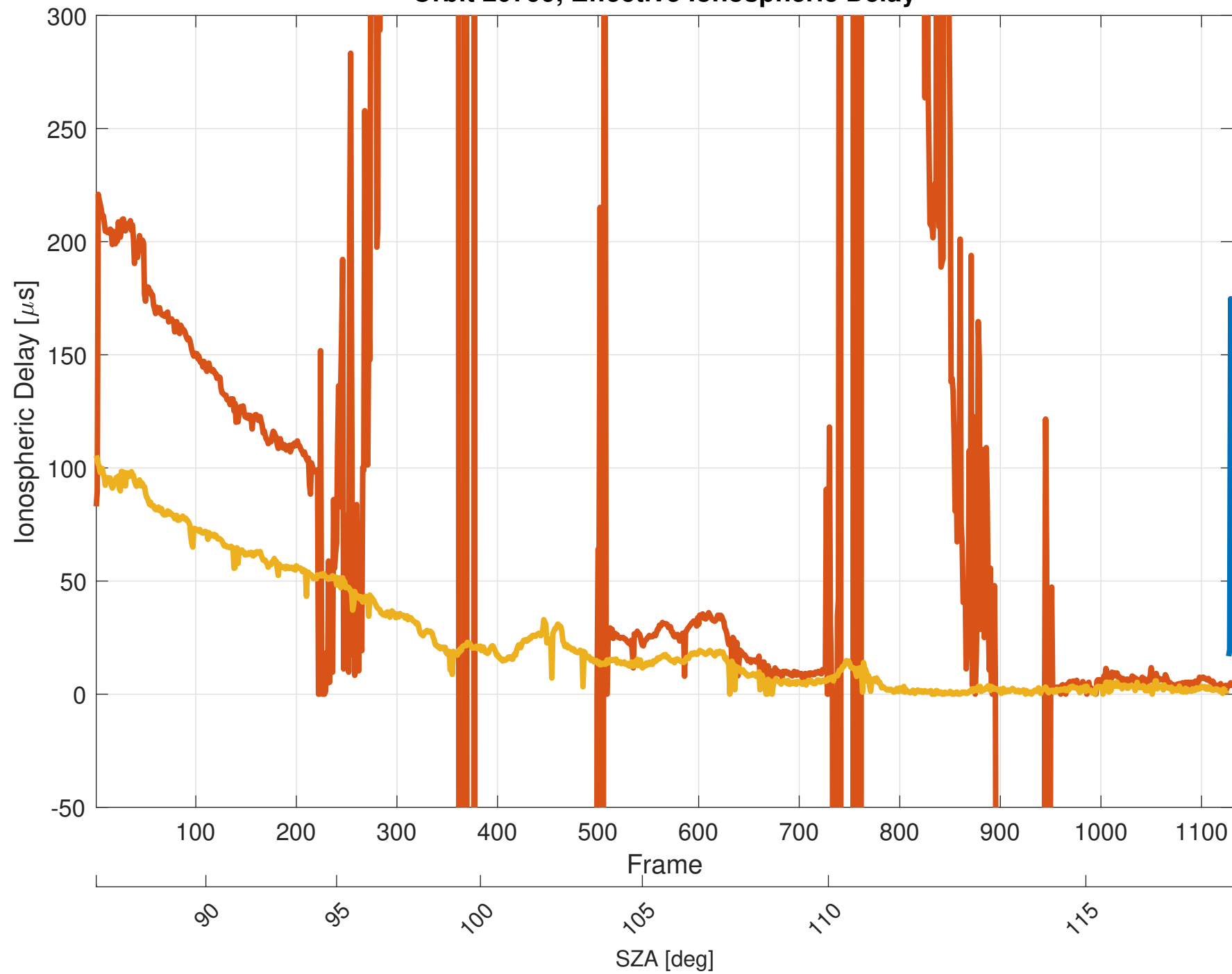
Orbit 20799, Effective Ionospheric Delay
