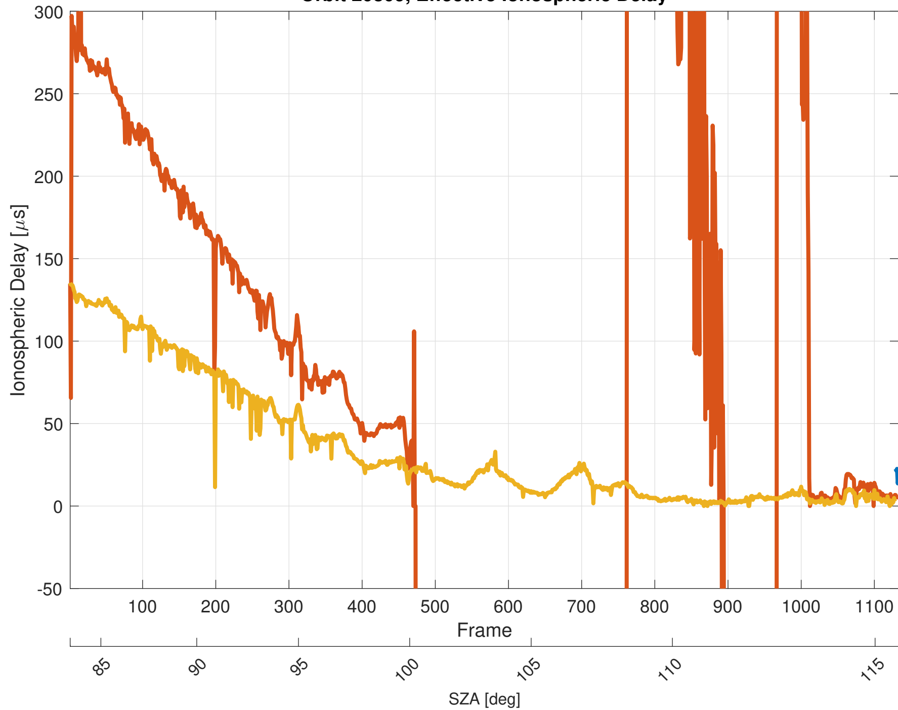
Orbit 20809, Effective Ionospheric Delay
