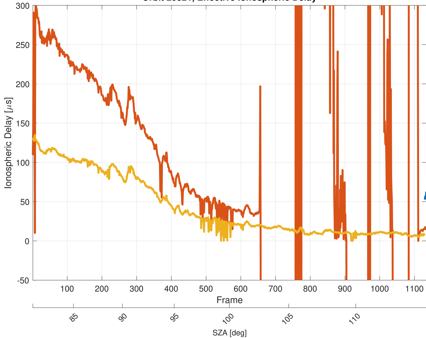
Orbit 20821, Effective Ionospheric Delay
