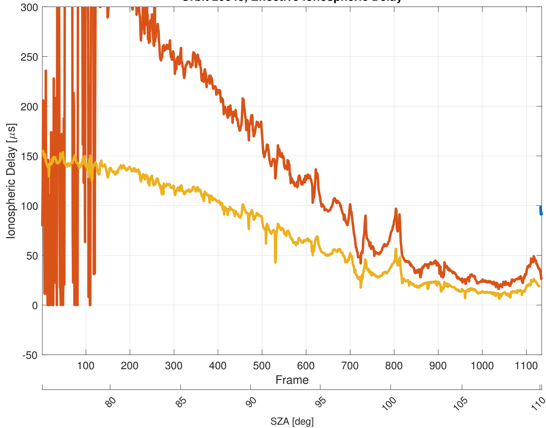
Orbit 20848, Effective Ionospheric Delay
