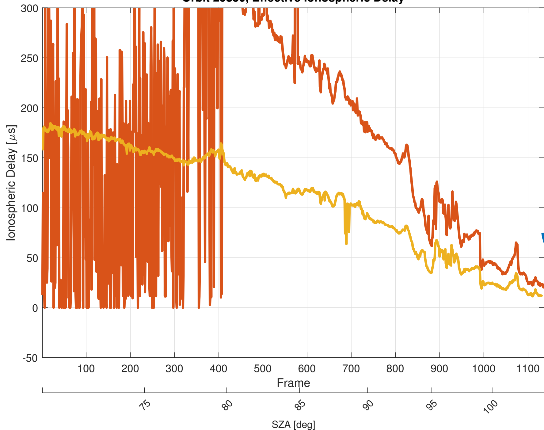
Orbit 20880, Effective Ionospheric Delay
