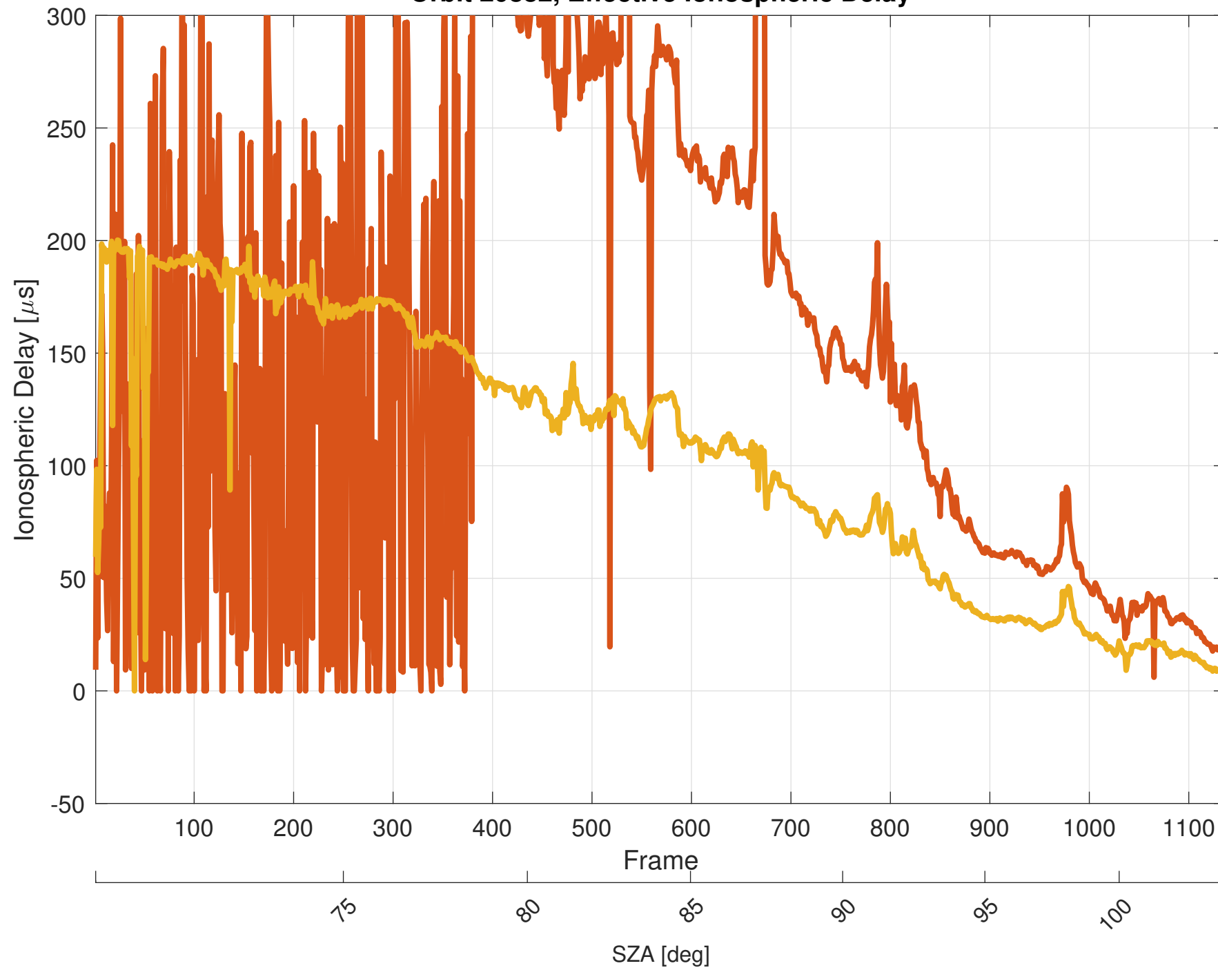
Orbit 20882, Effective Ionospheric Delay
