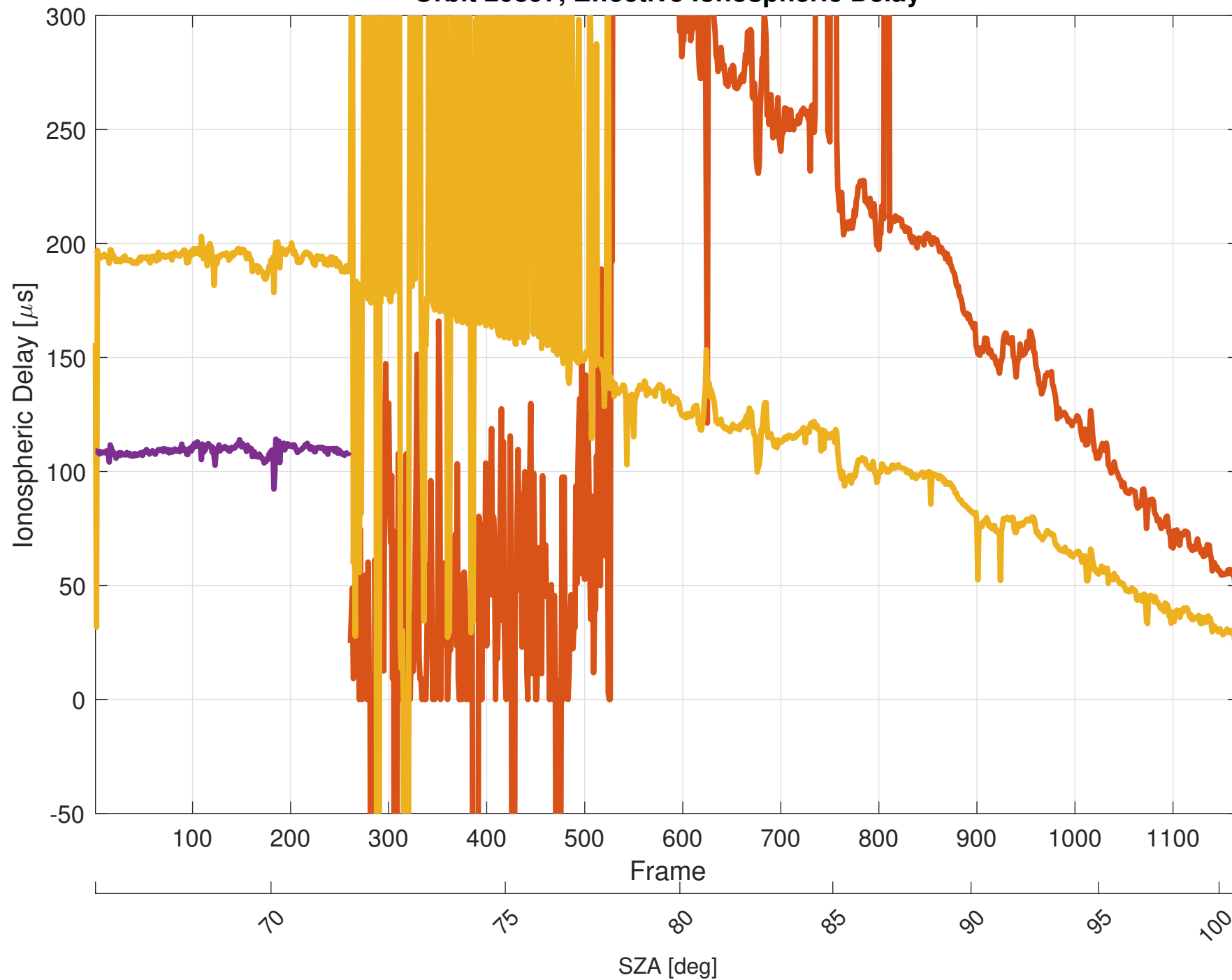
Orbit 20897, Effective Ionospheric Delay
