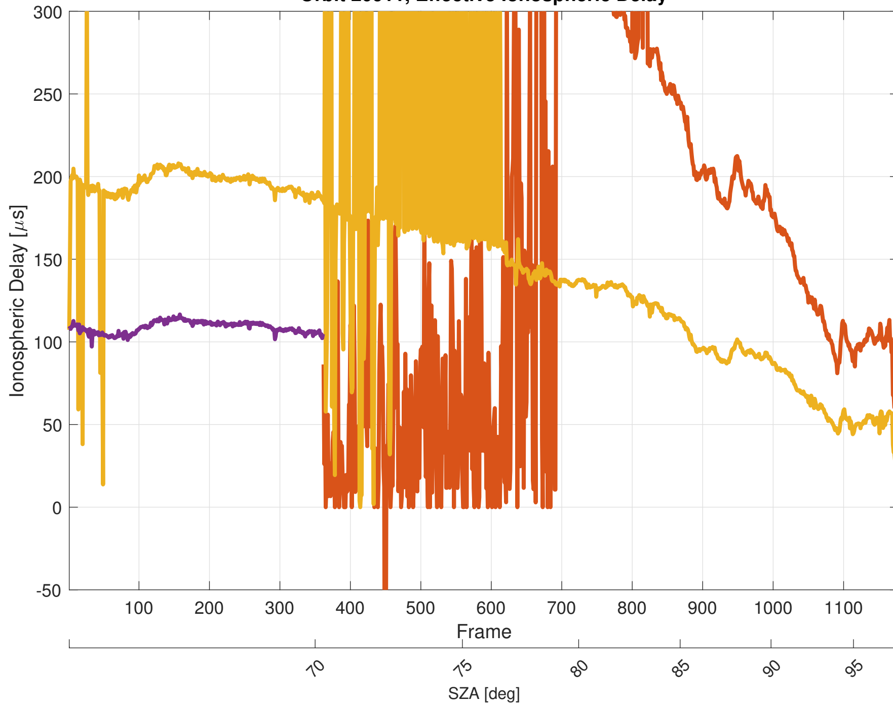
Orbit 20911, Effective Ionospheric Delay
