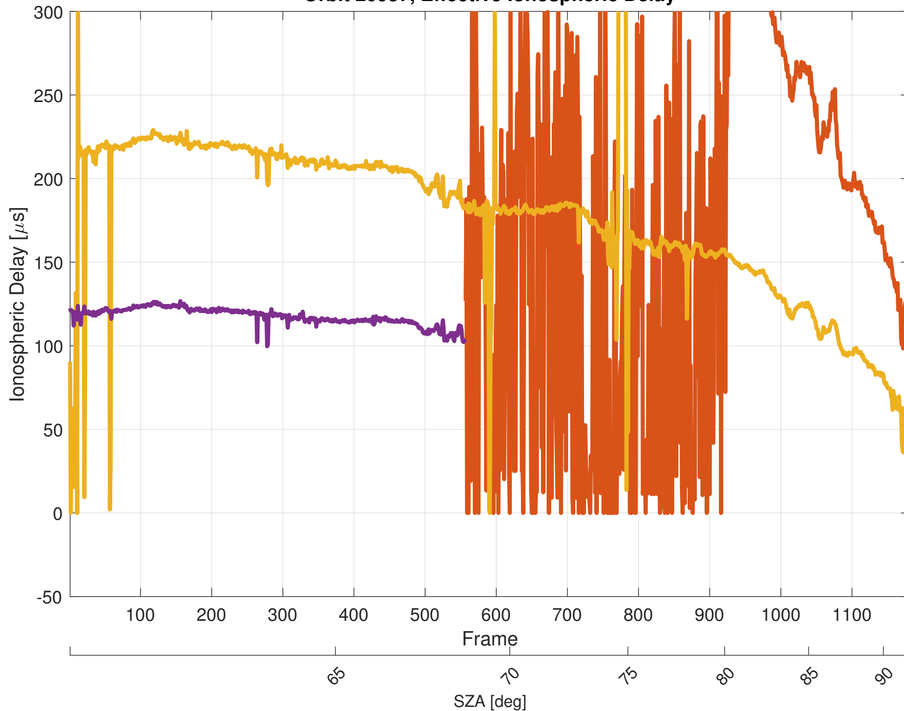
Orbit 20937, Effective Ionospheric Delay
