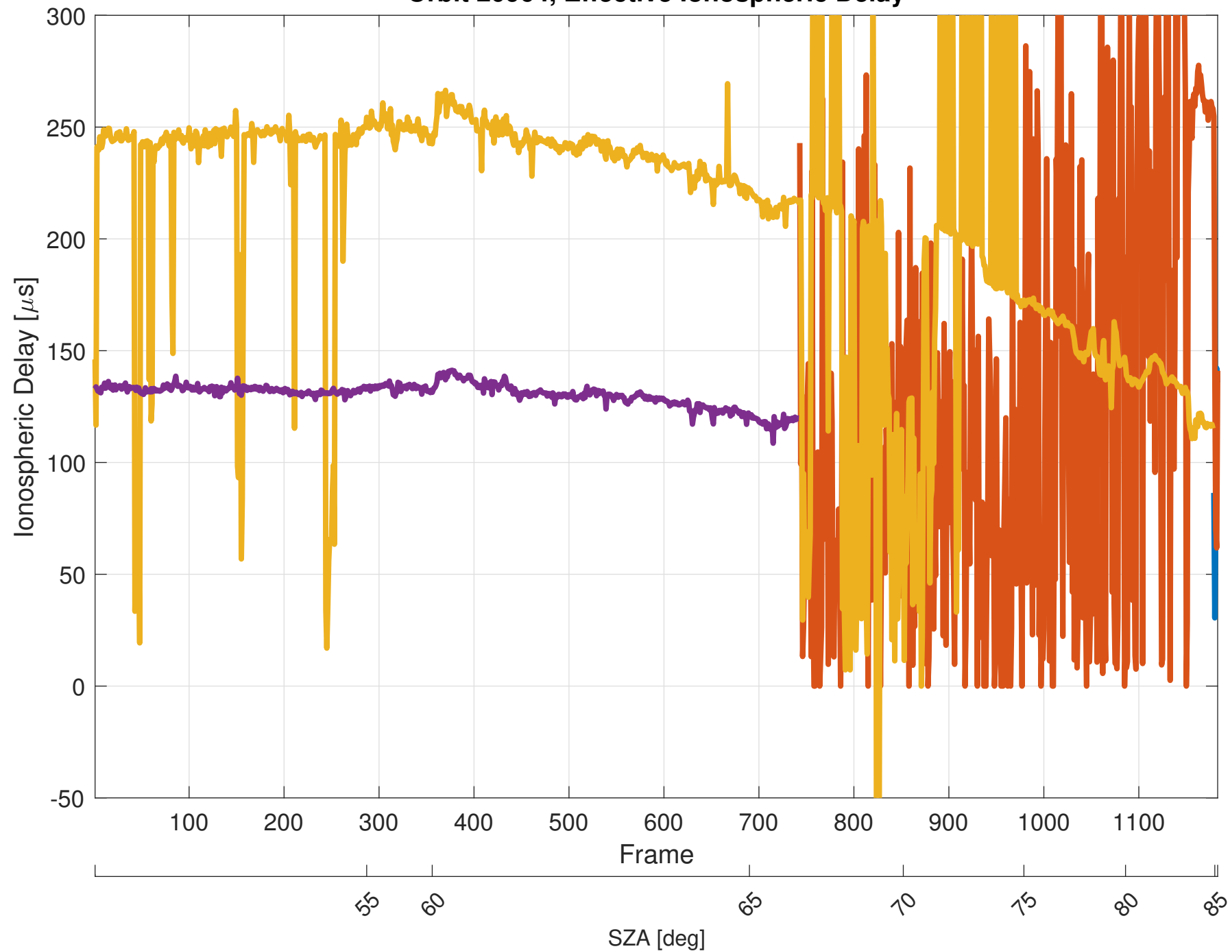
Orbit 20964, Effective Ionospheric Delay
