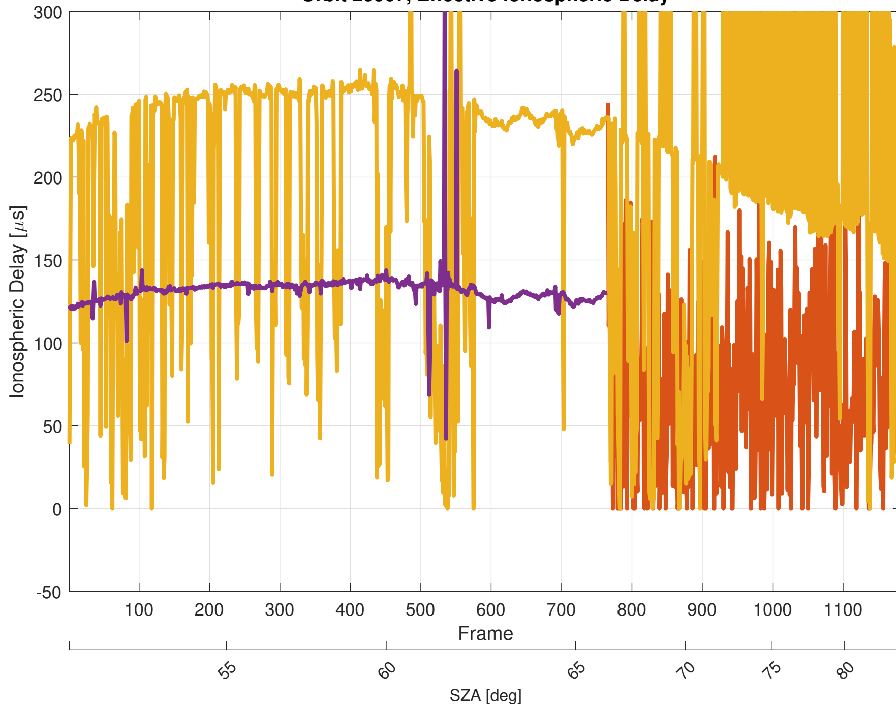
Orbit 20967, Effective Ionospheric Delay
