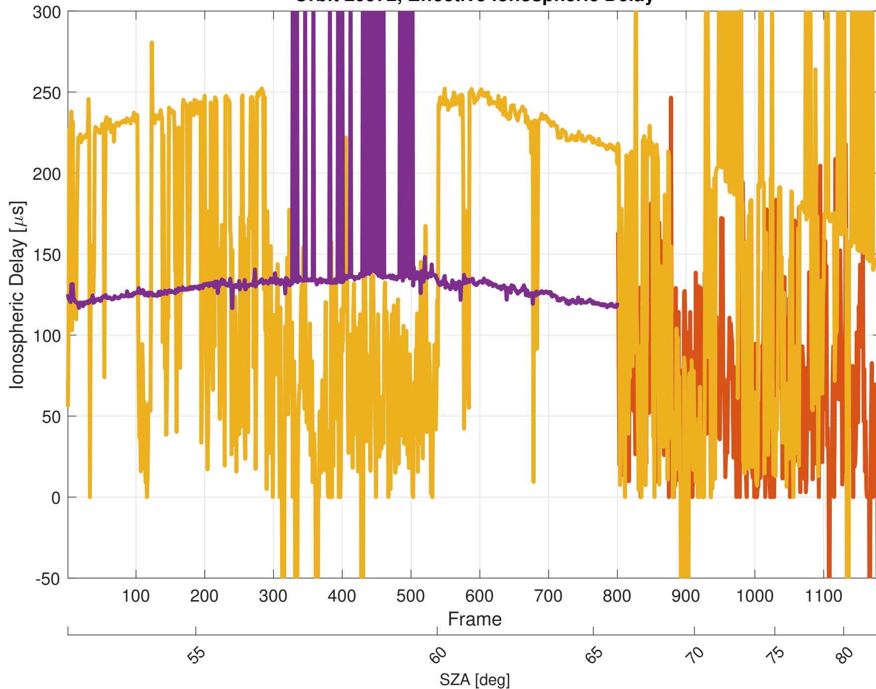
Orbit 20972, Effective Ionospheric Delay
