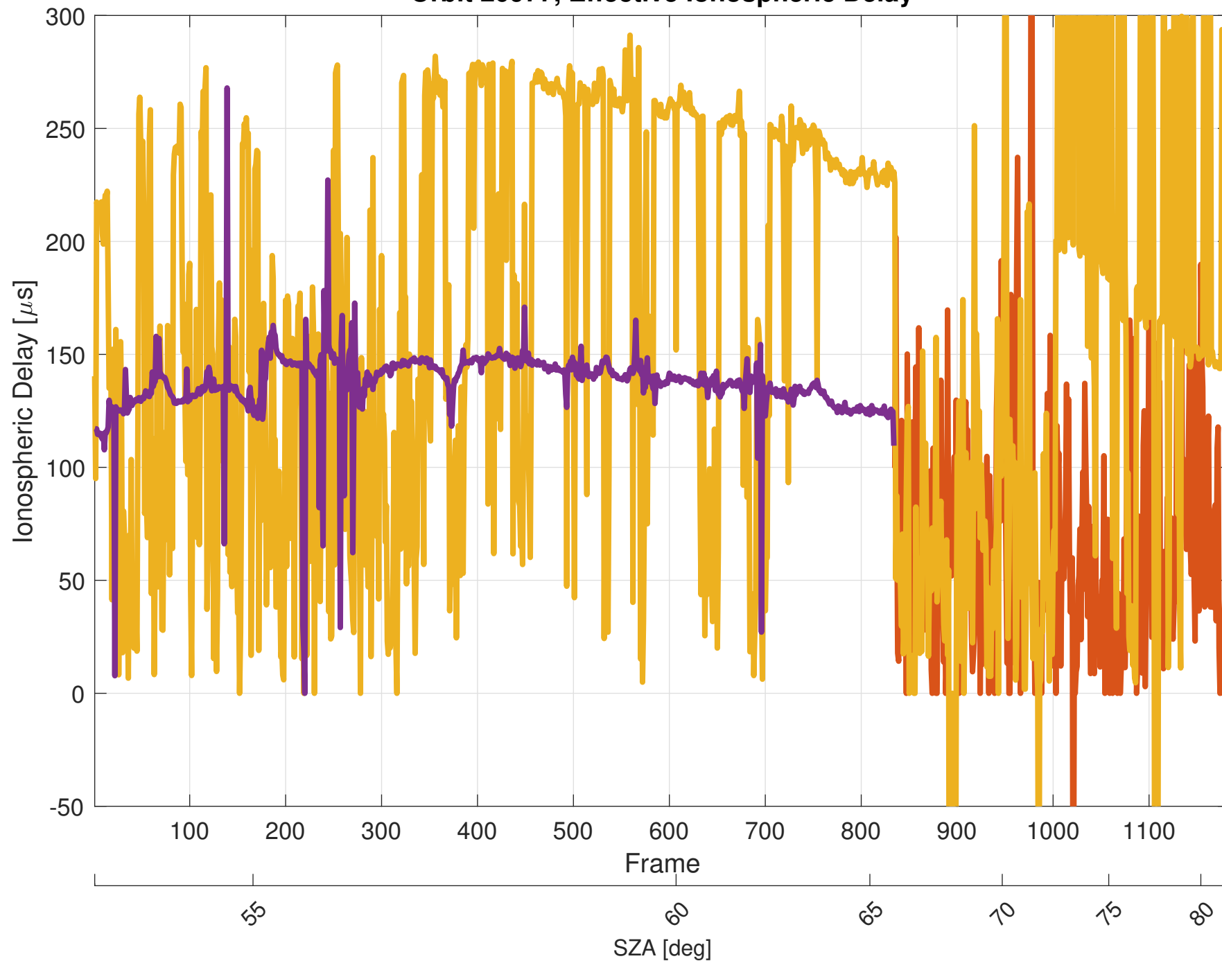
Orbit 20977, Effective Ionospheric Delay
