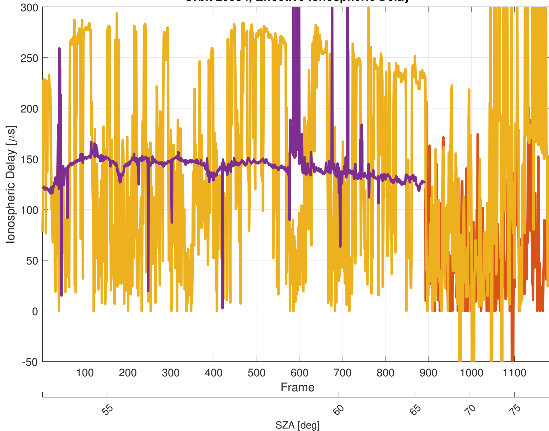
Orbit 20984, Effective Ionospheric Delay
