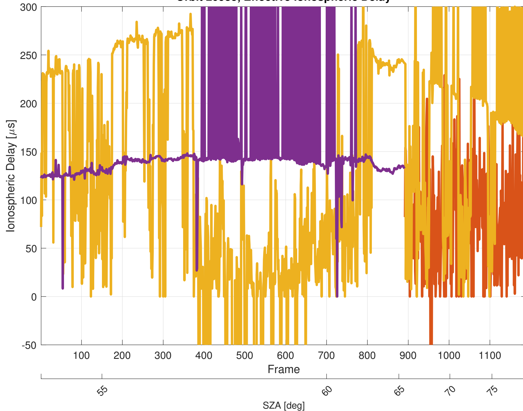
Orbit 20985, Effective Ionospheric Delay
