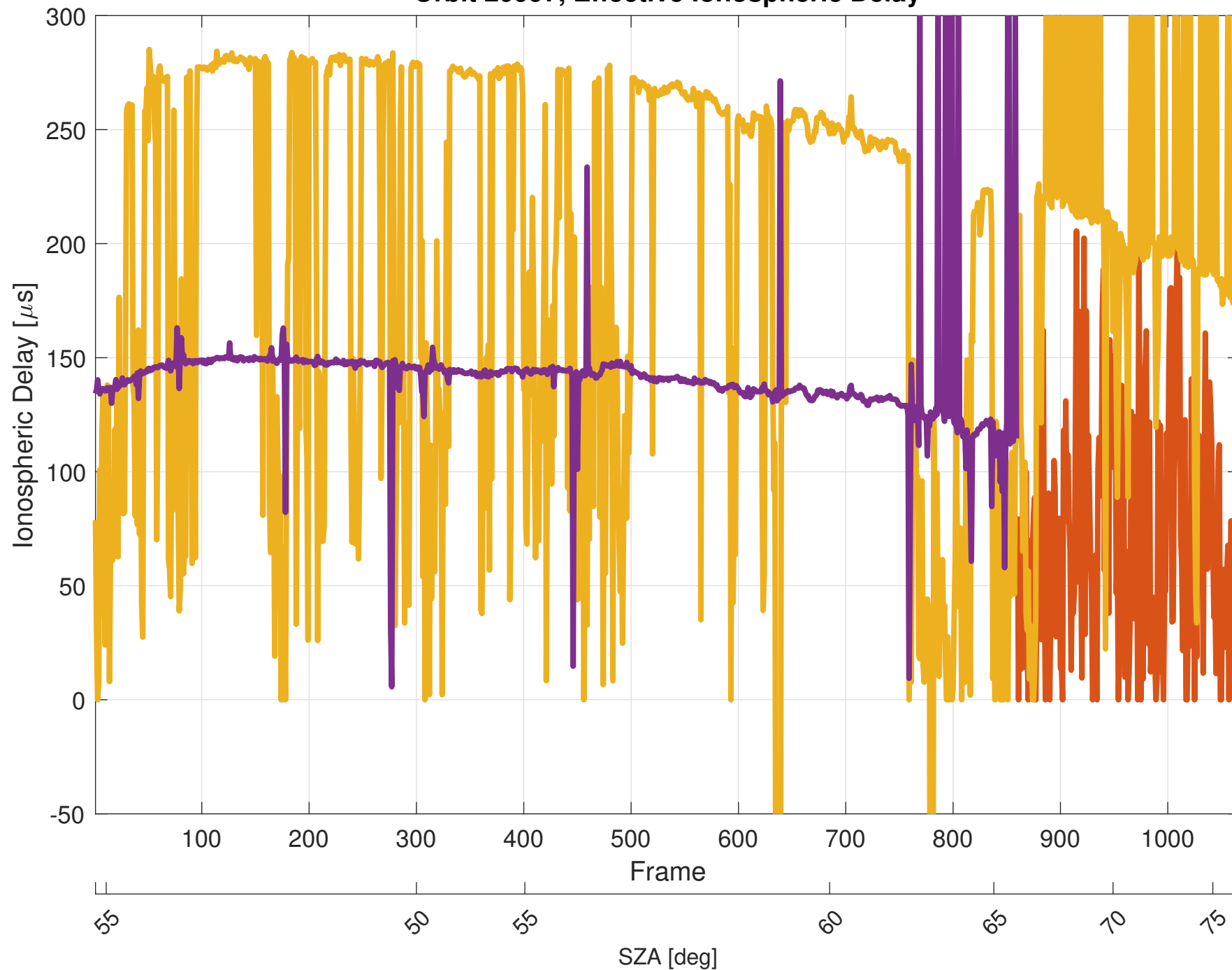
Orbit 20997, Effective Ionospheric Delay
