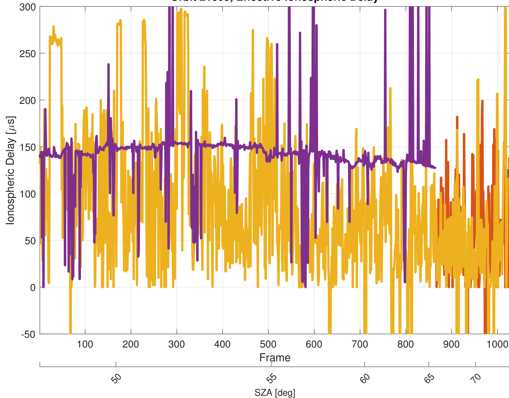
Orbit 21005, Effective Ionospheric Delay
