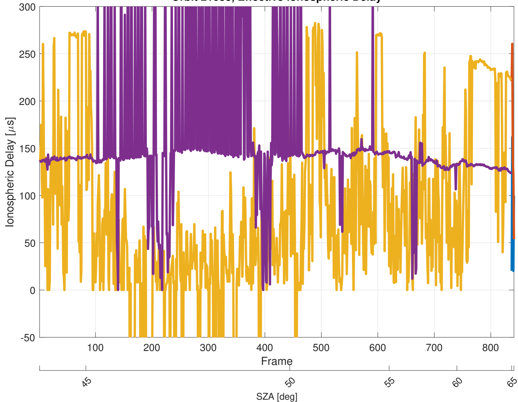
Orbit 21038, Effective Ionospheric Delay
