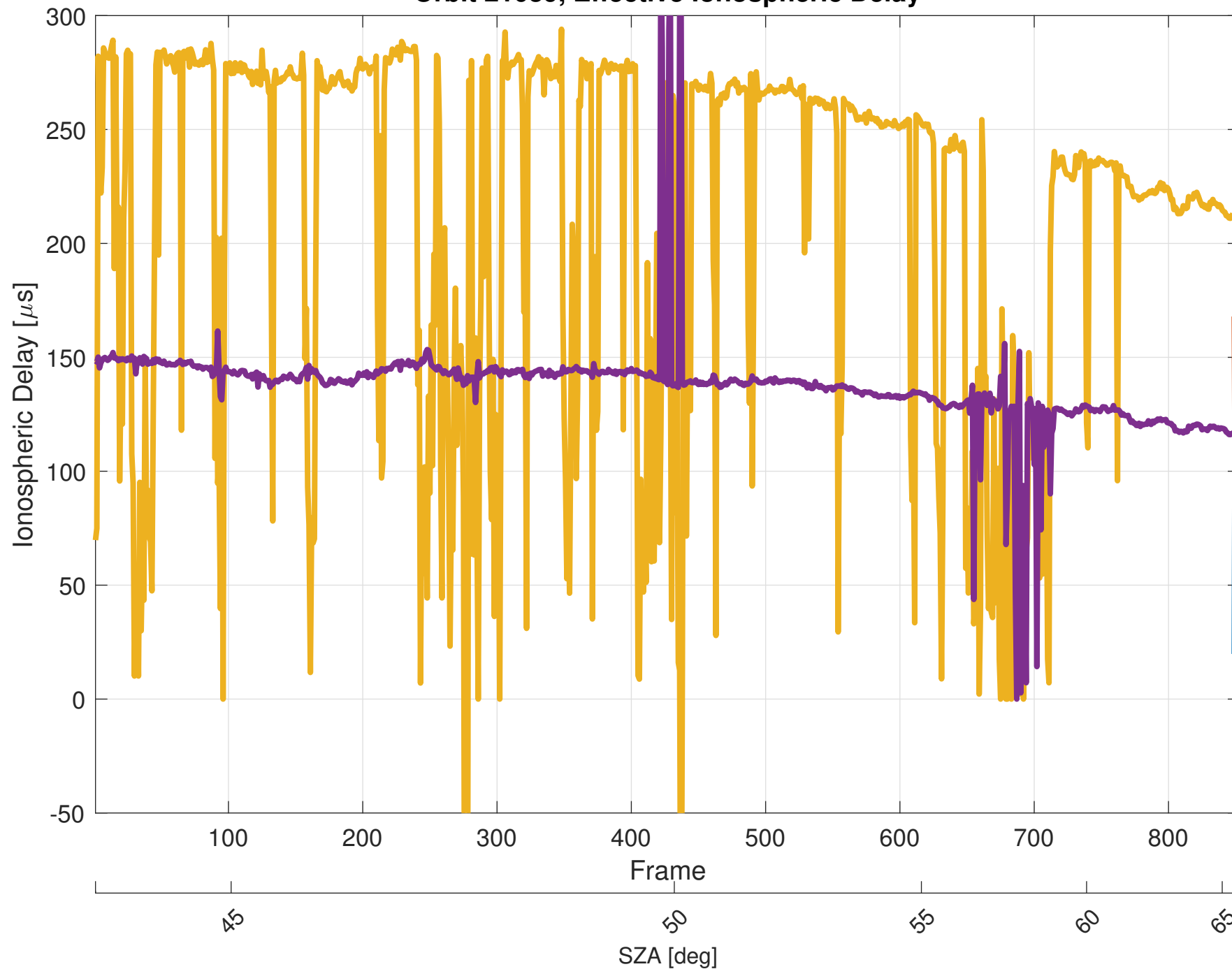
Orbit 21039, Effective Ionospheric Delay
