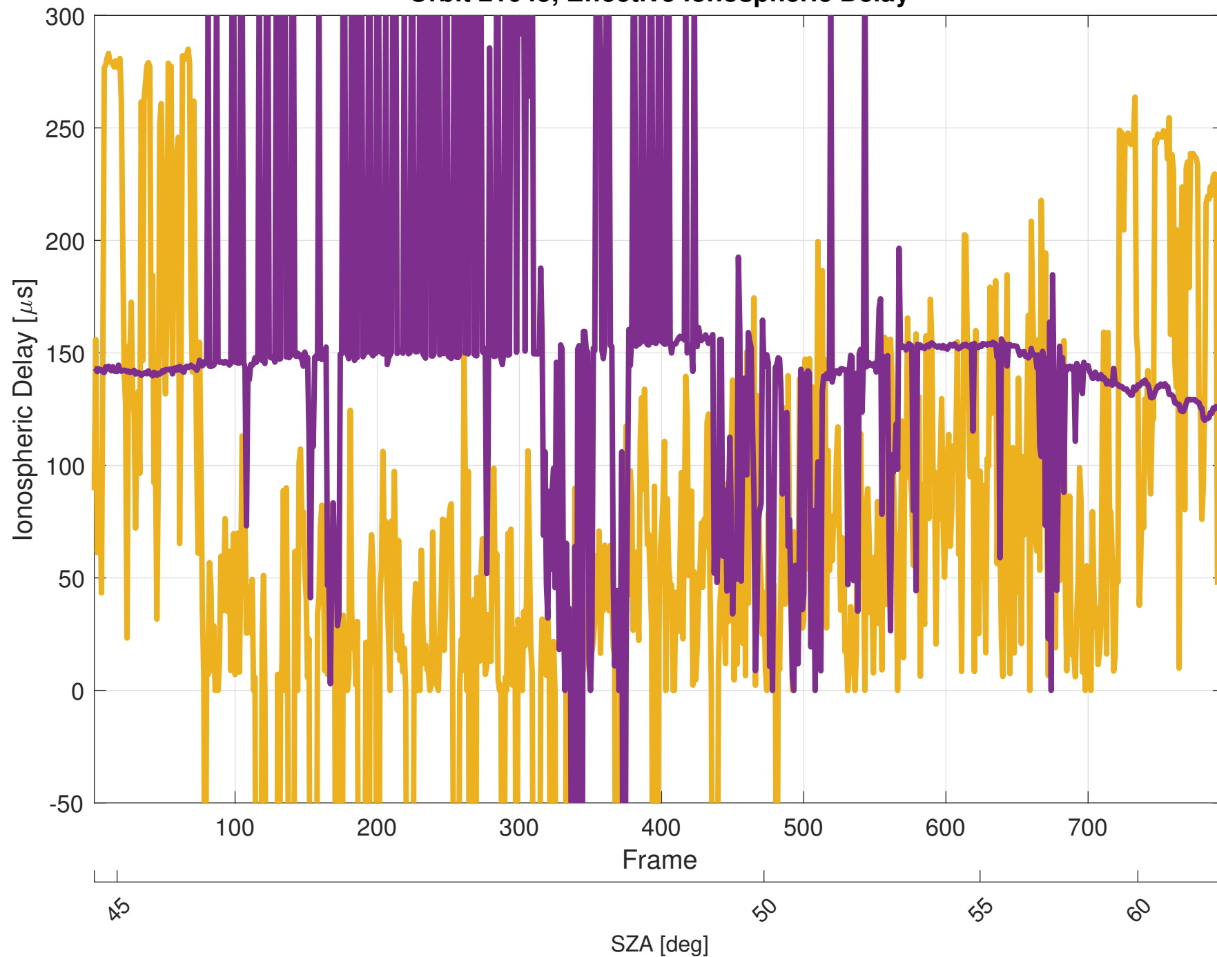
Orbit 21045, Effective Ionospheric Delay
