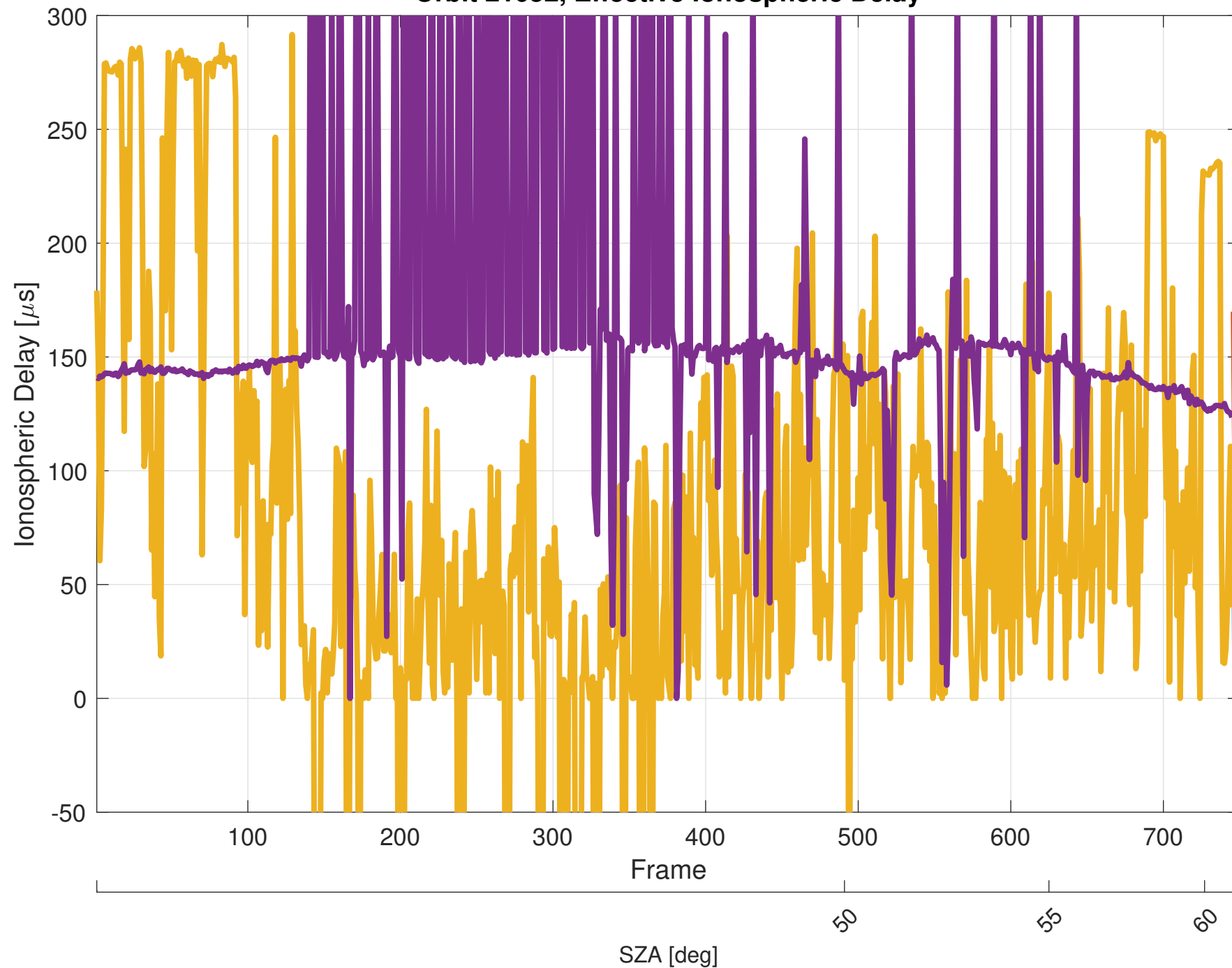
Orbit 21052, Effective Ionospheric Delay
