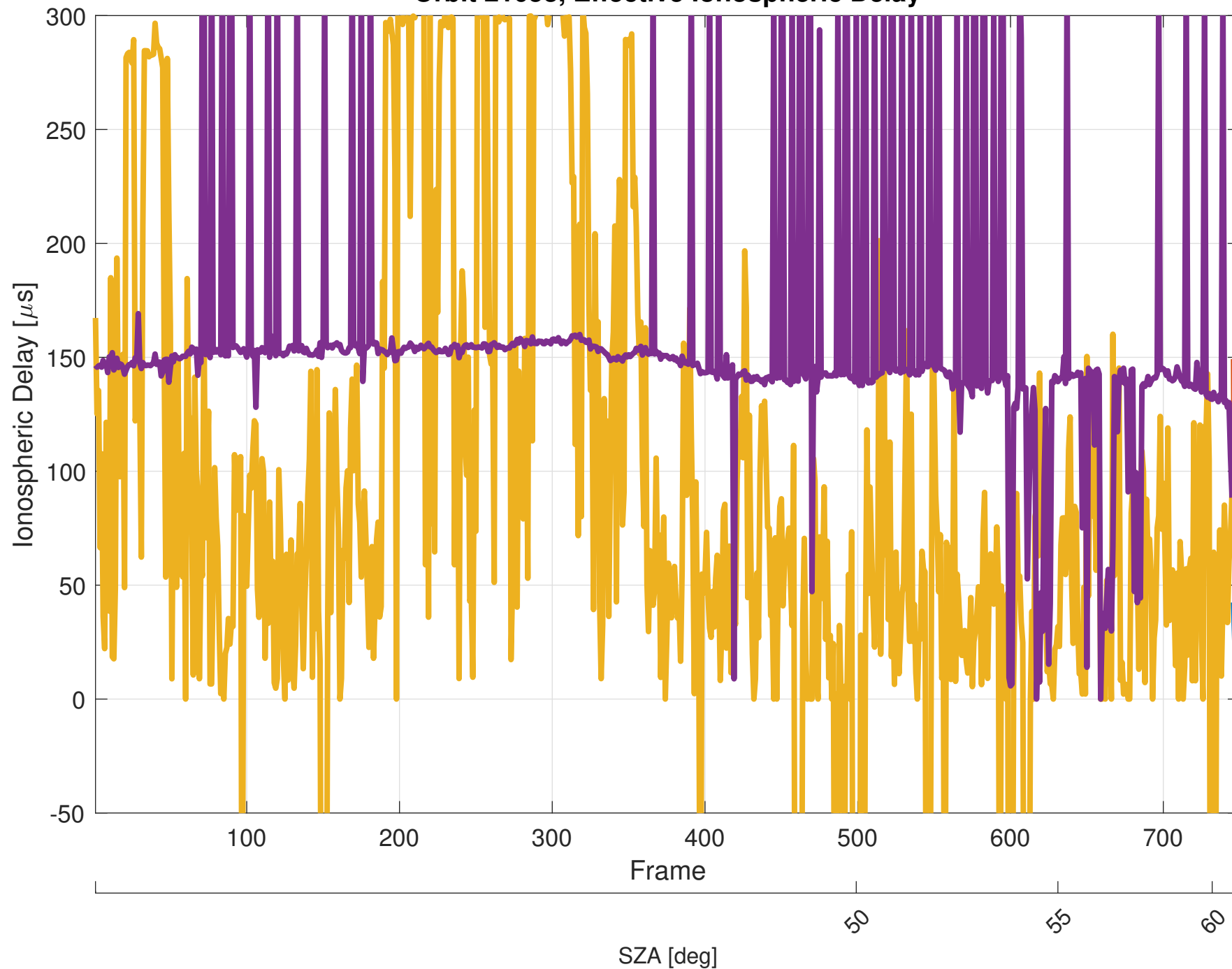
Orbit 21053, Effective Ionospheric Delay
