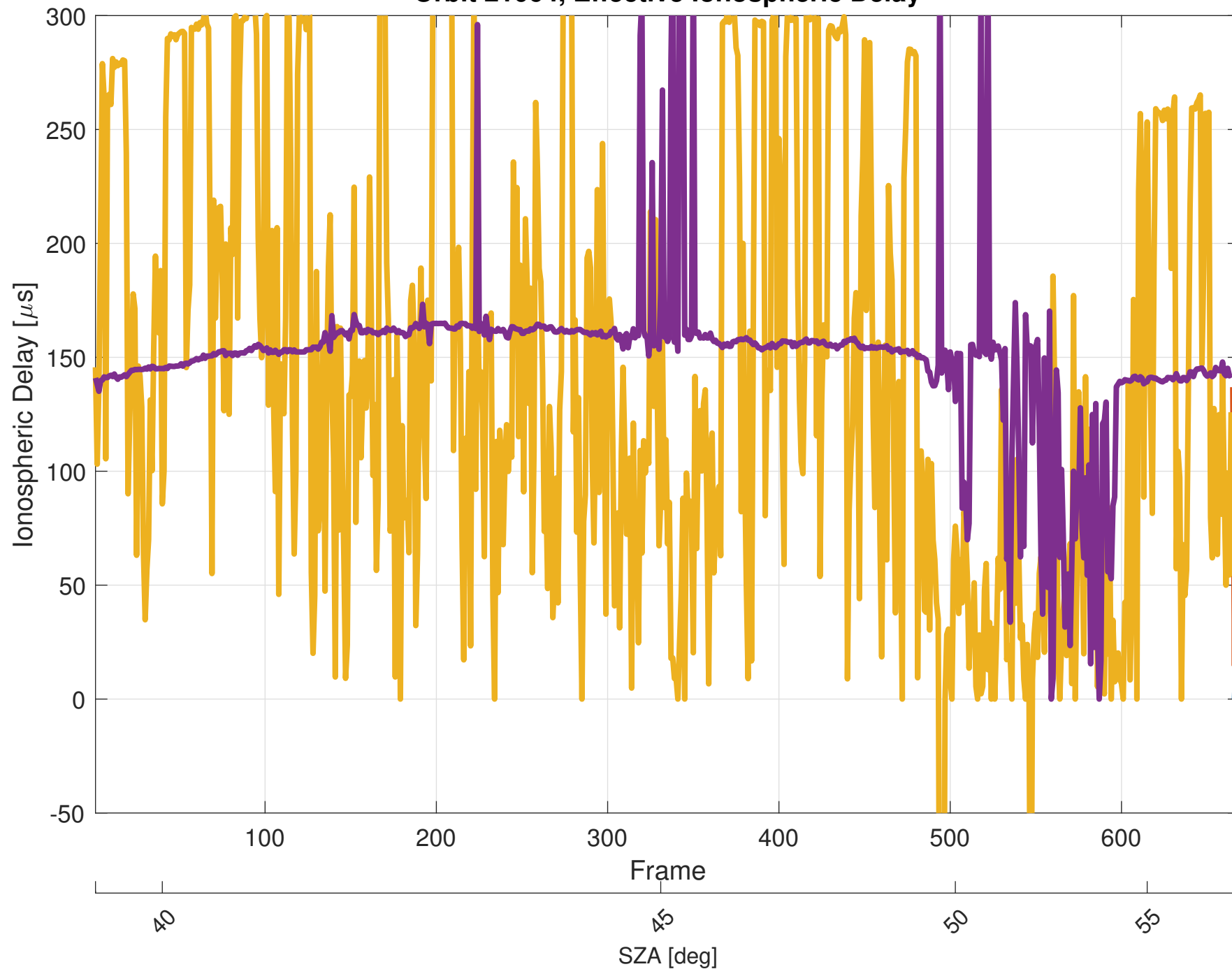
Orbit 21064, Effective Ionospheric Delay
