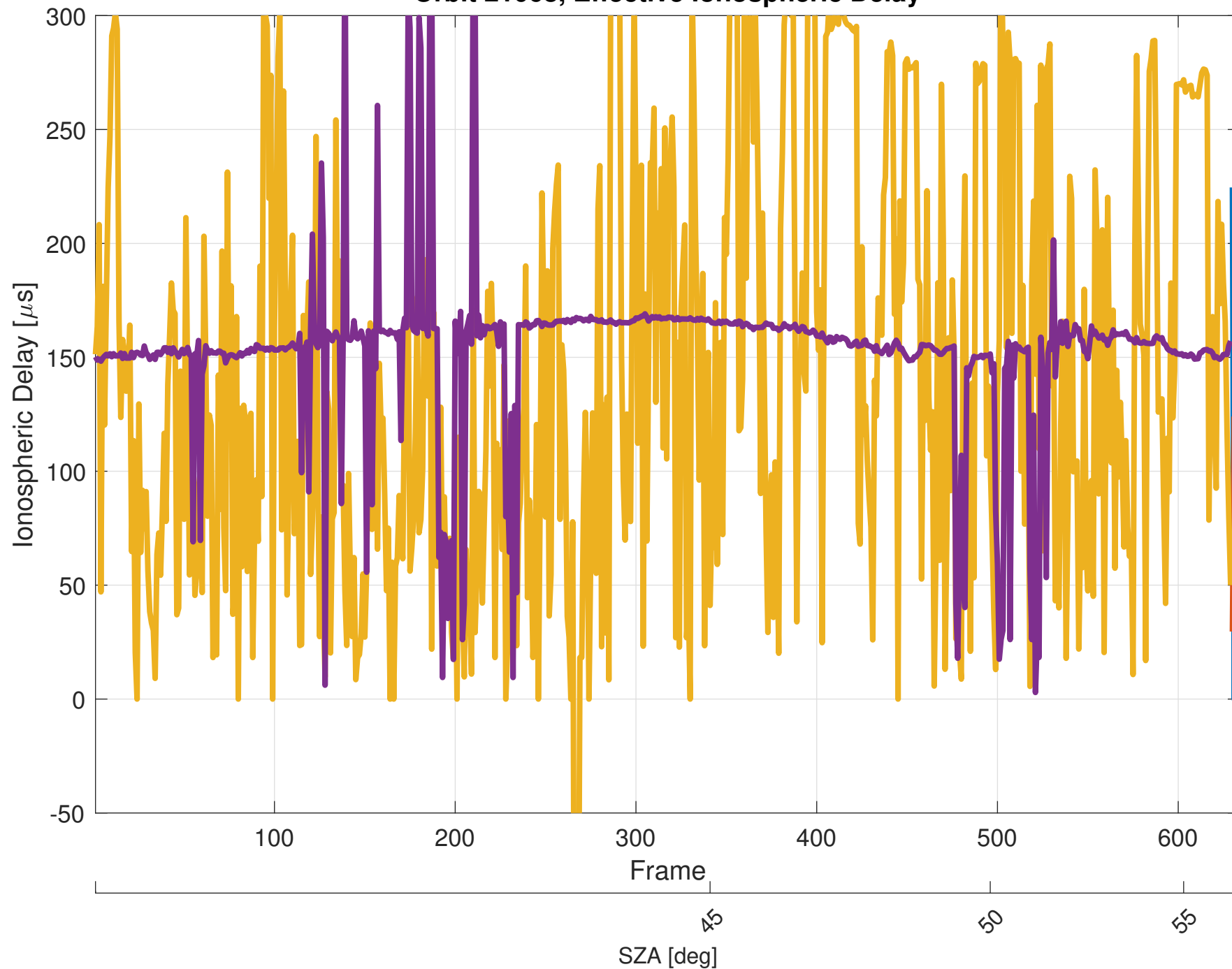
Orbit 21068, Effective Ionospheric Delay
