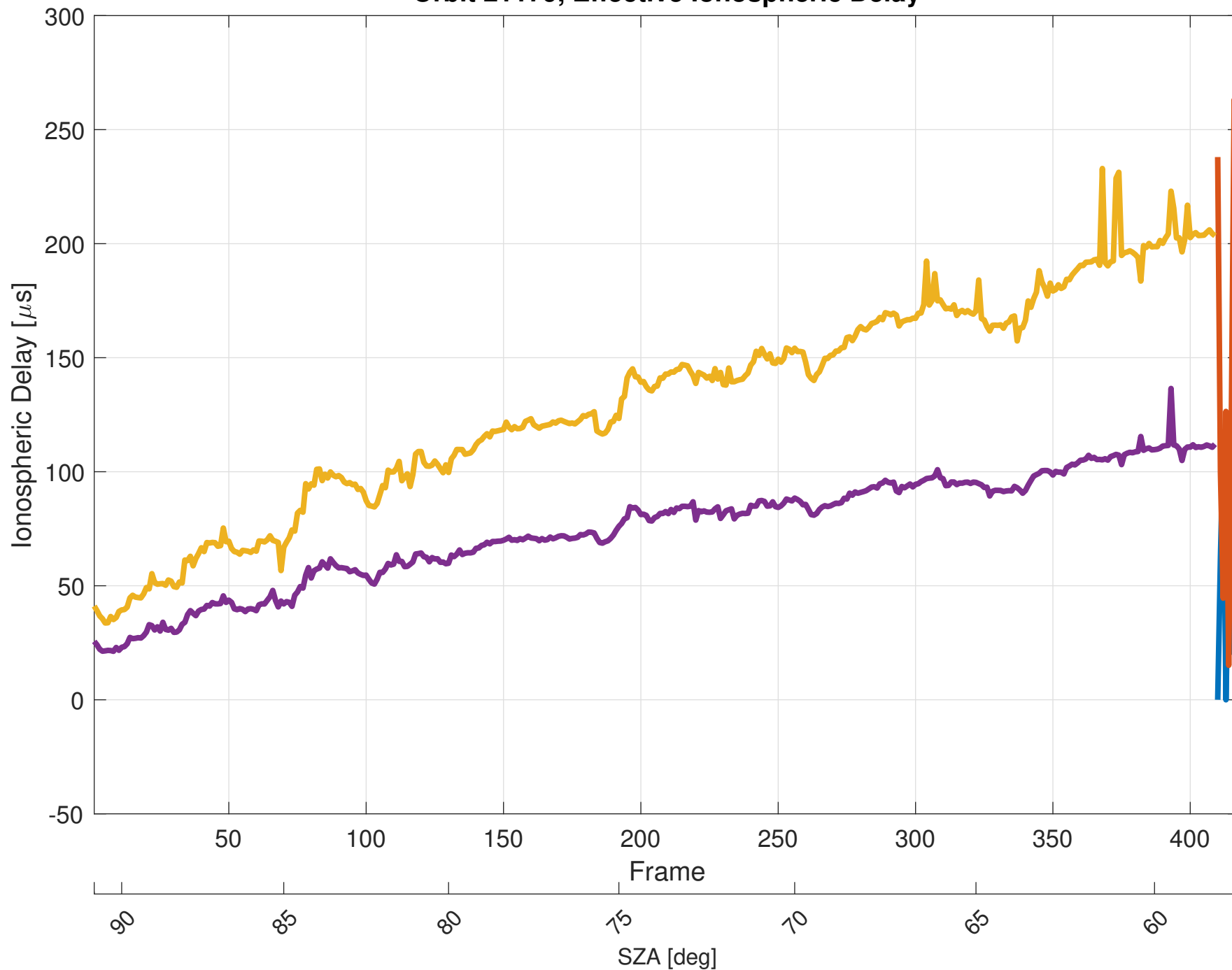
Orbit 21179, Effective Ionospheric Delay
