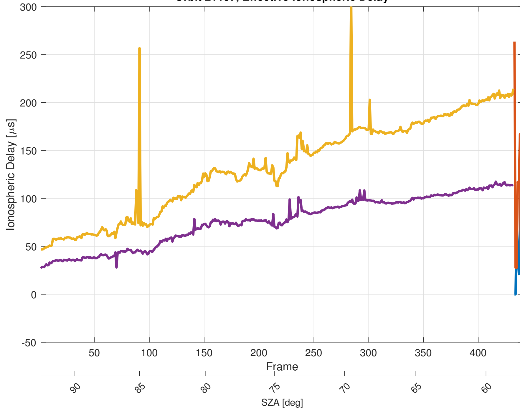
Orbit 21187, Effective Ionospheric Delay
