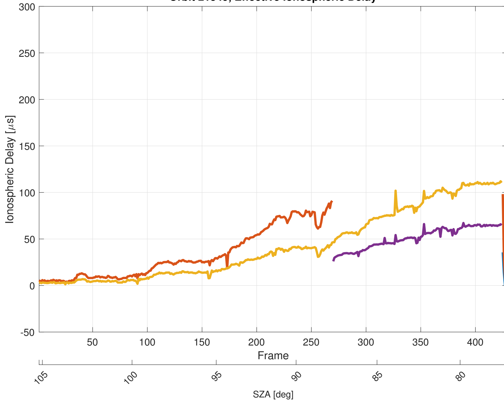
Orbit 21549, Effective Ionospheric Delay
