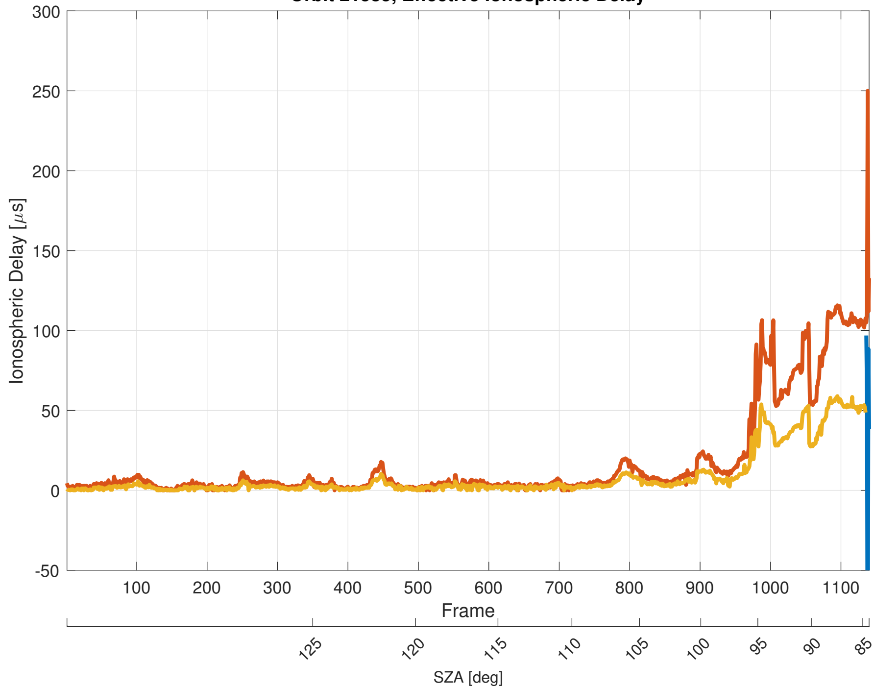
Orbit 21585, Effective Ionospheric Delay
