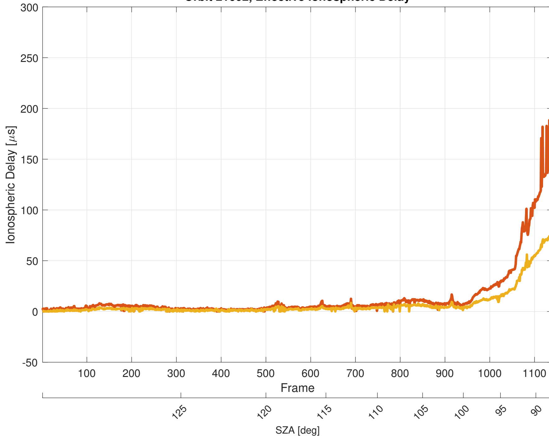
Orbit 21602, Effective Ionospheric Delay
