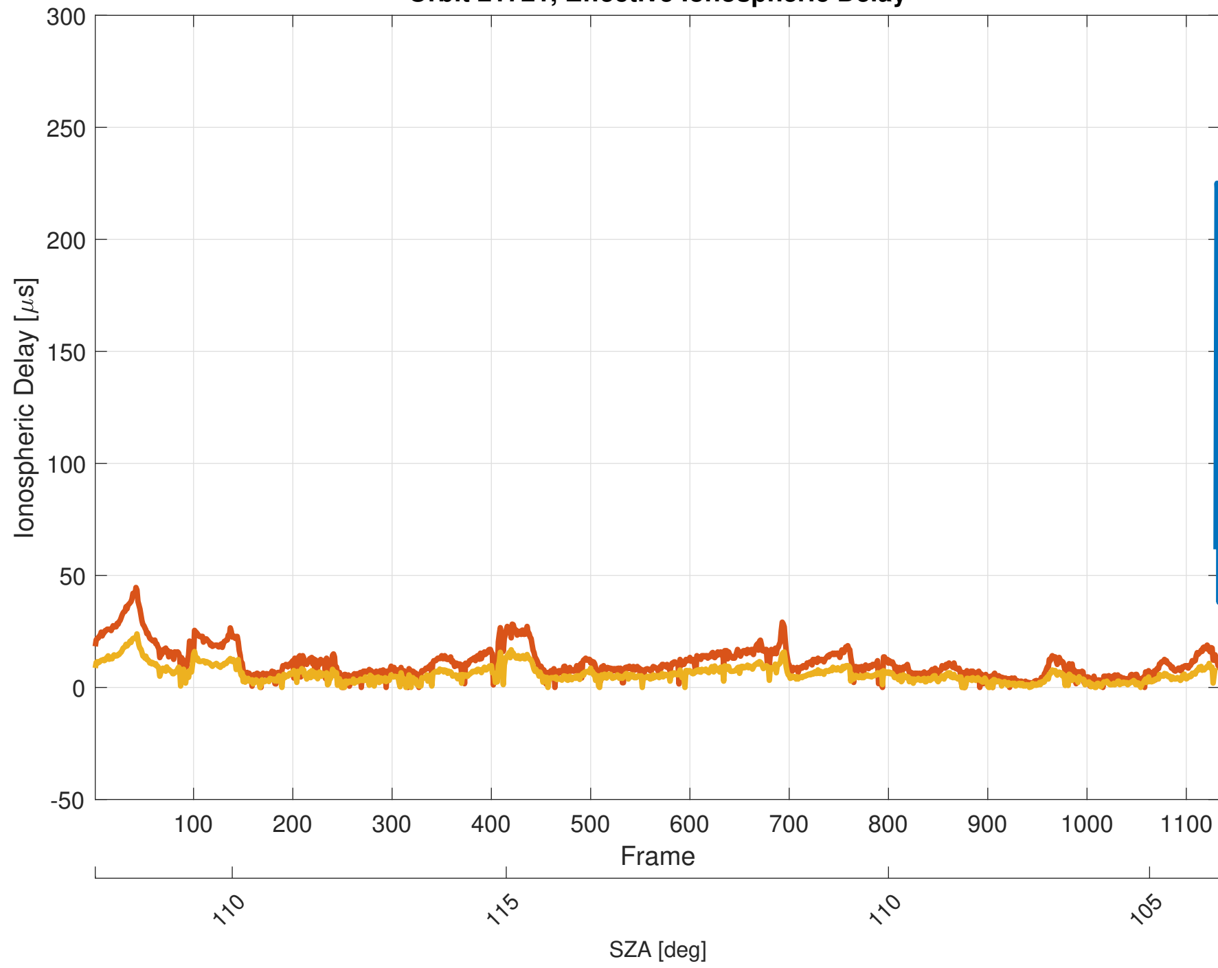
Orbit 21721, Effective Ionospheric Delay
