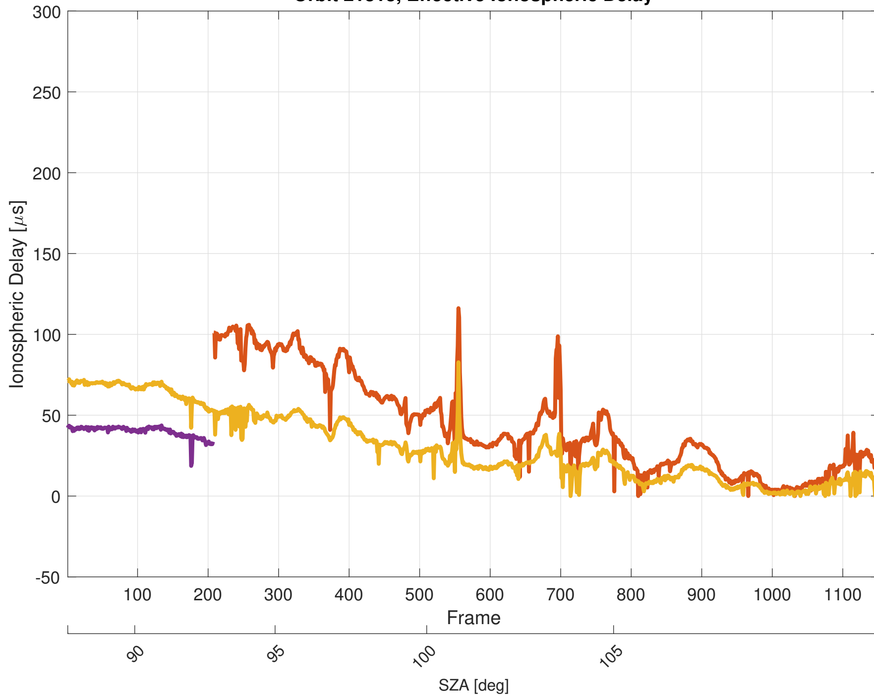
Orbit 21813, Effective Ionospheric Delay
