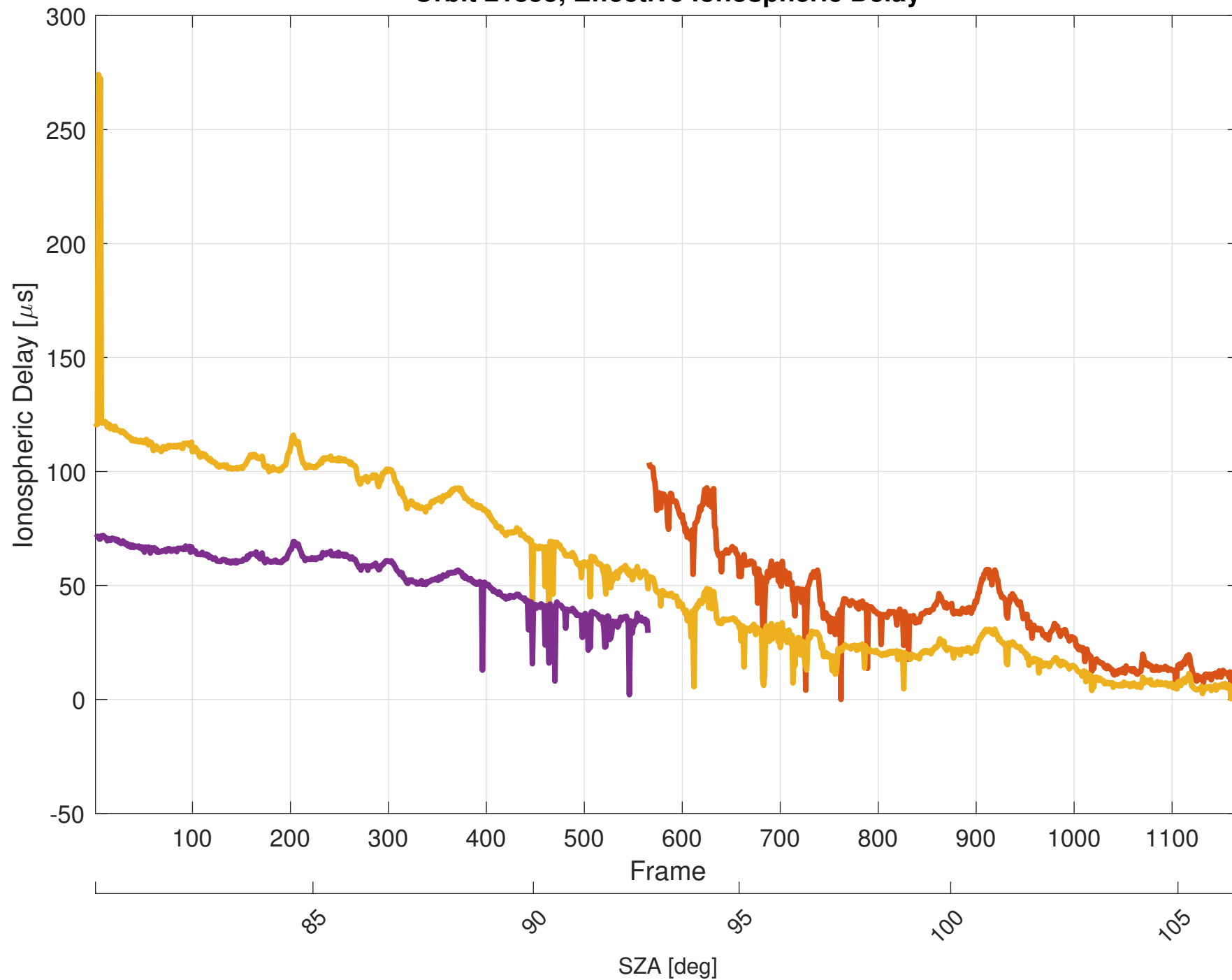
Orbit 21855, Effective Ionospheric Delay
