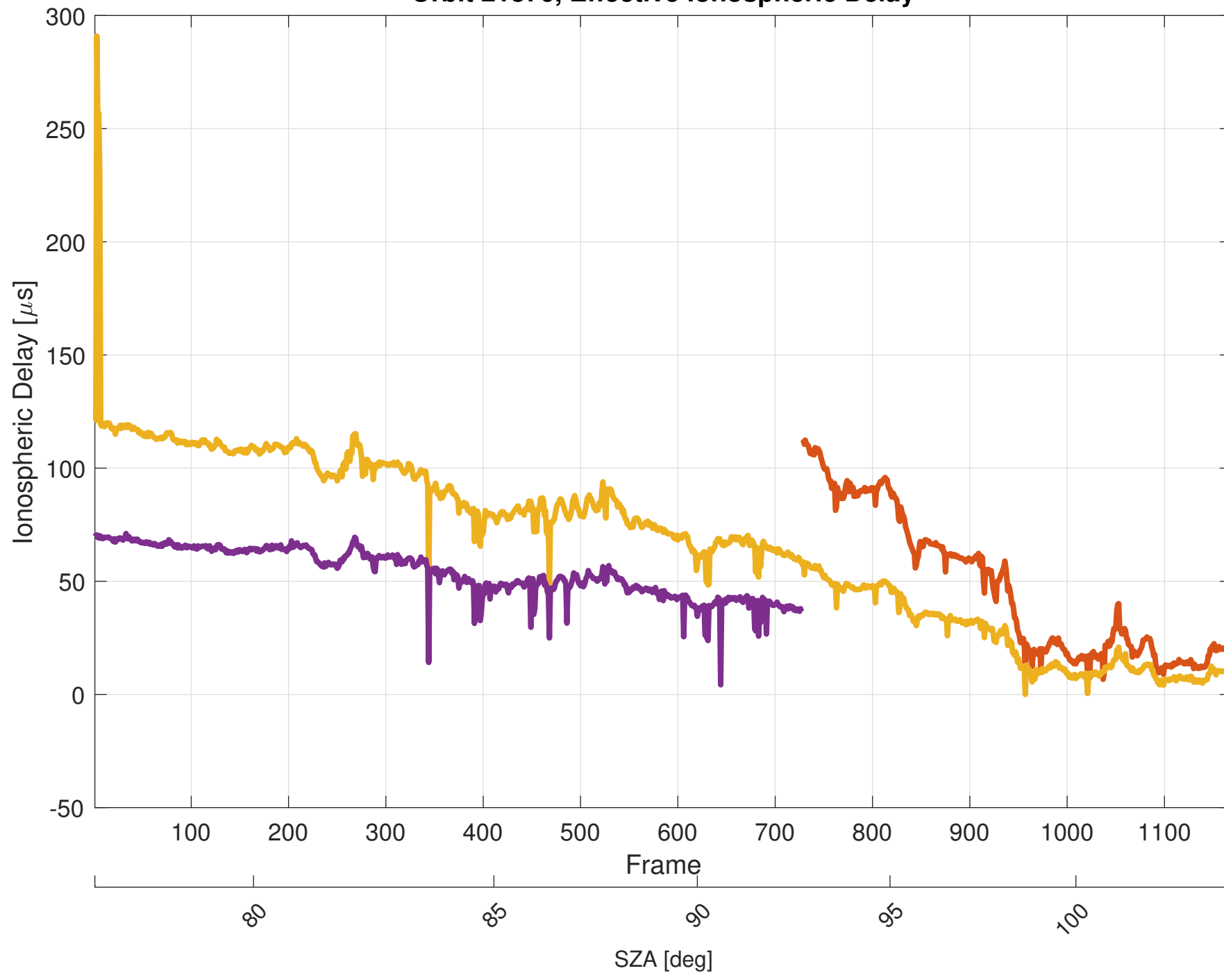
Orbit 21876, Effective Ionospheric Delay
