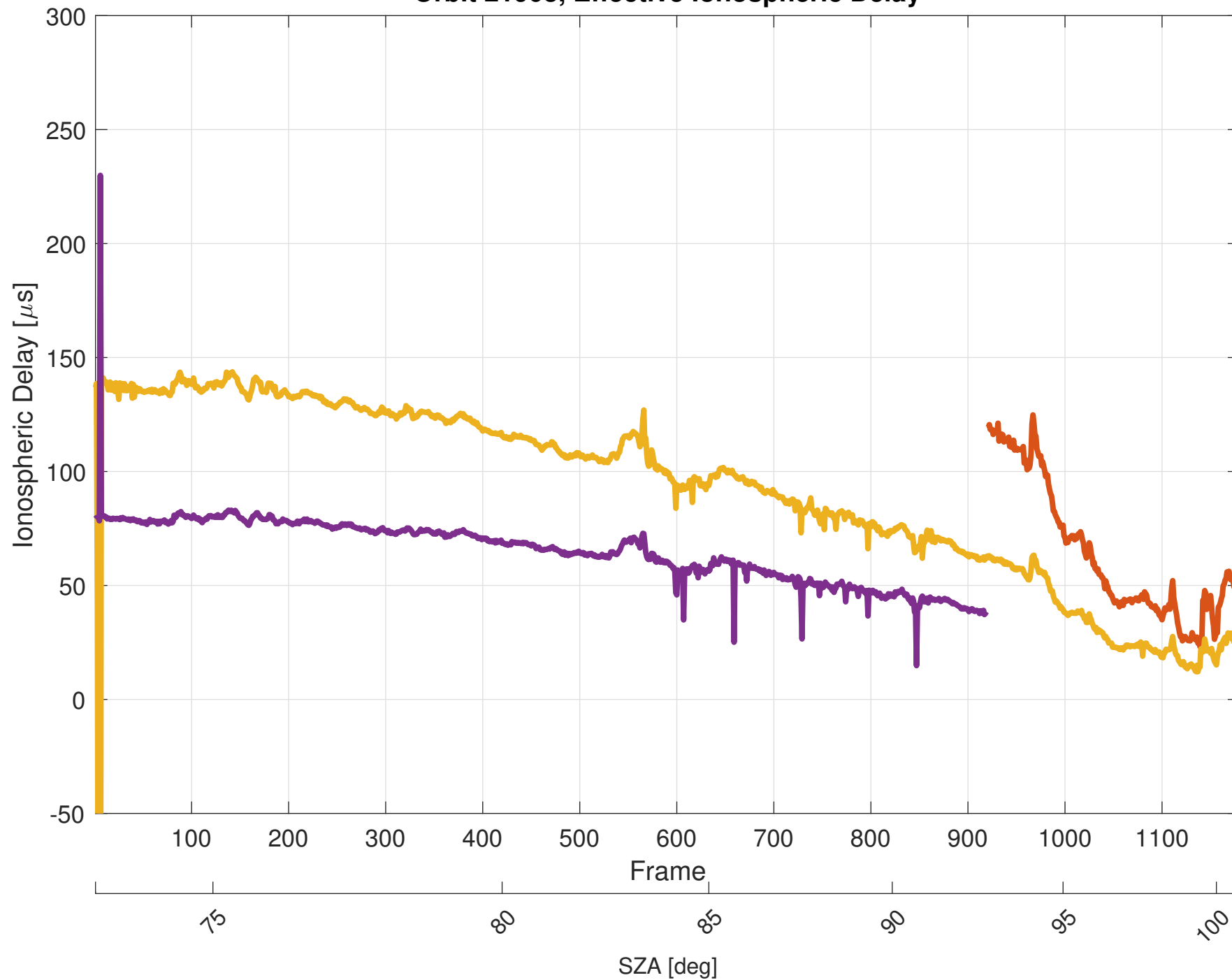
Orbit 21903, Effective Ionospheric Delay
