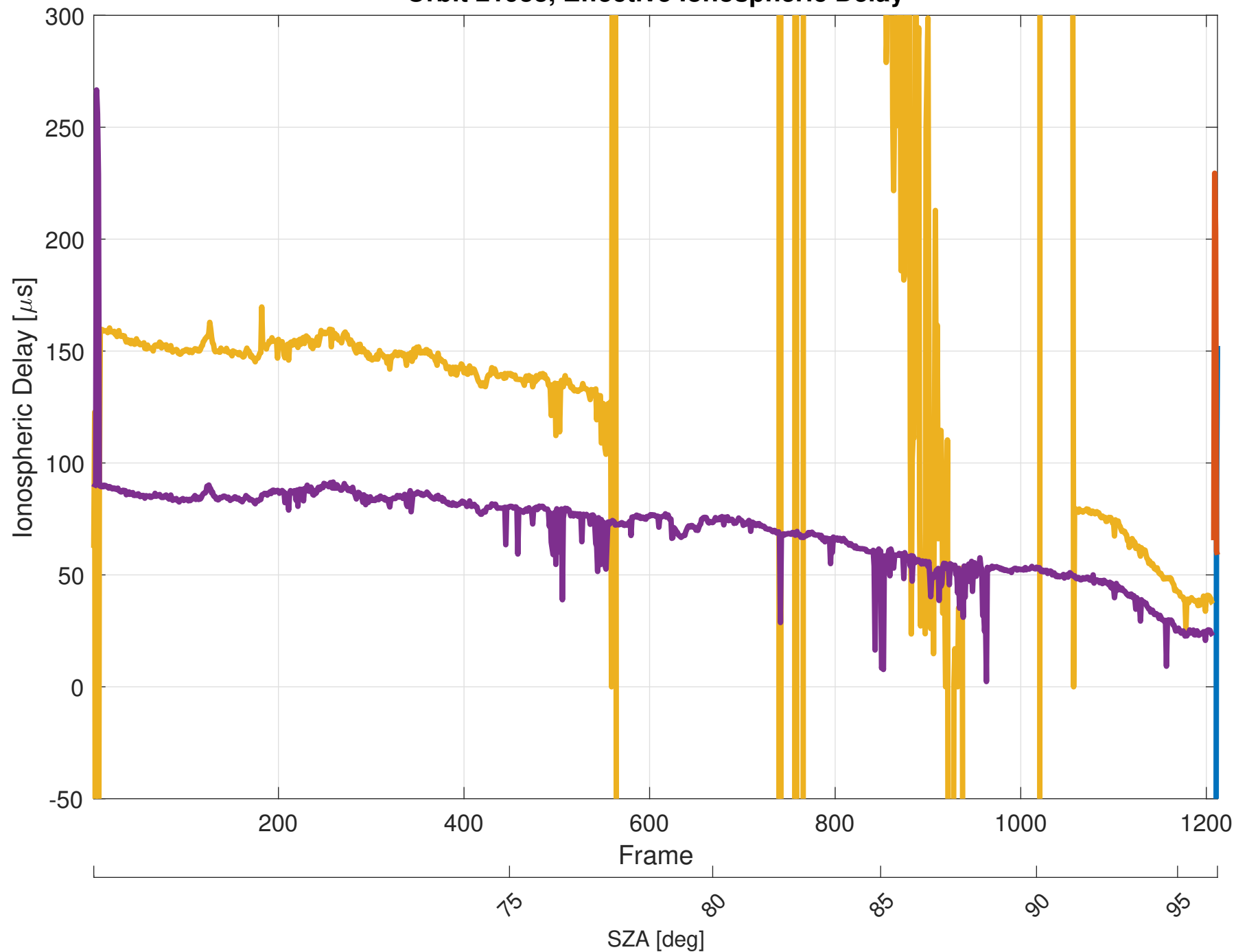
Orbit 21933, Effective Ionospheric Delay
