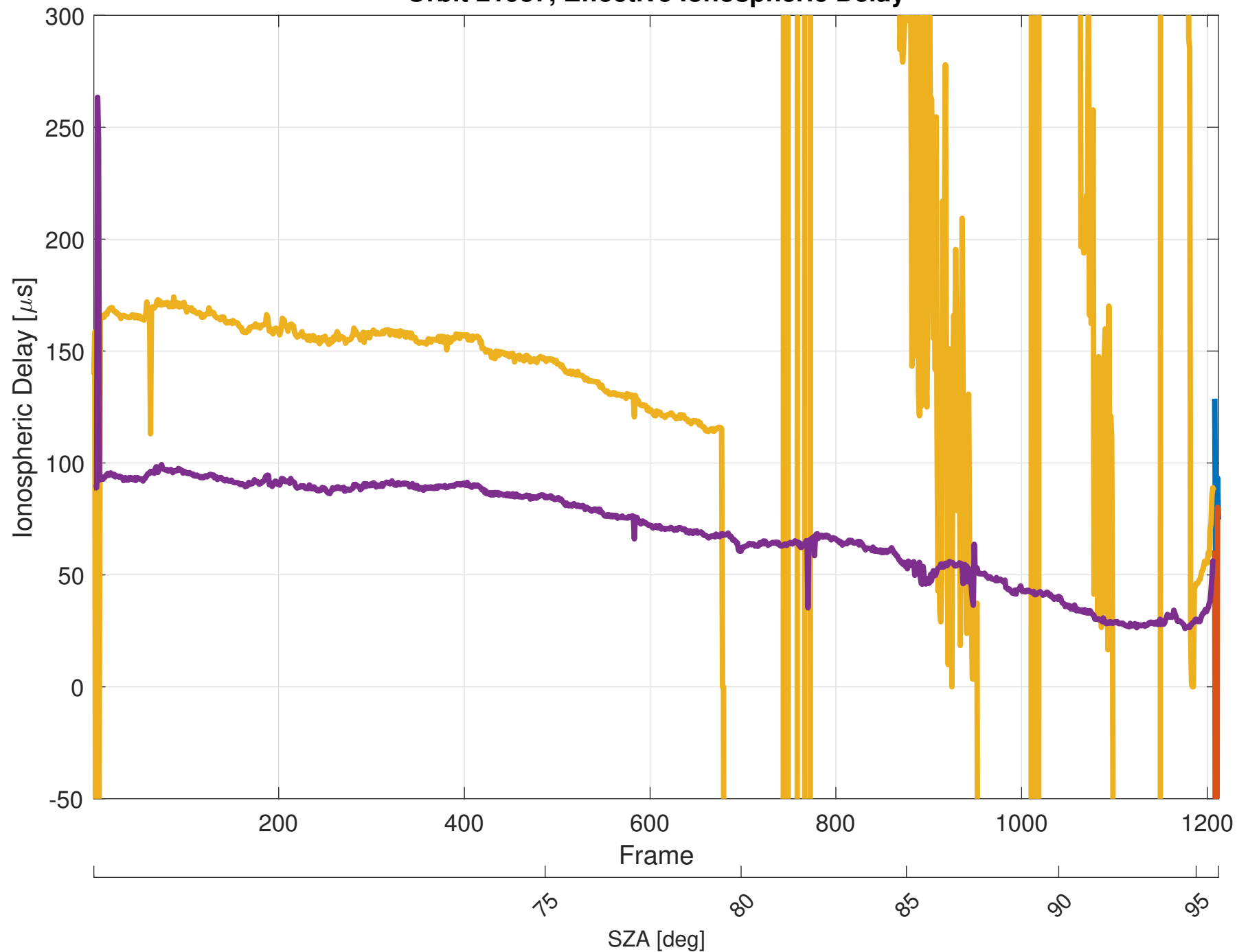
Orbit 21937, Effective Ionospheric Delay
