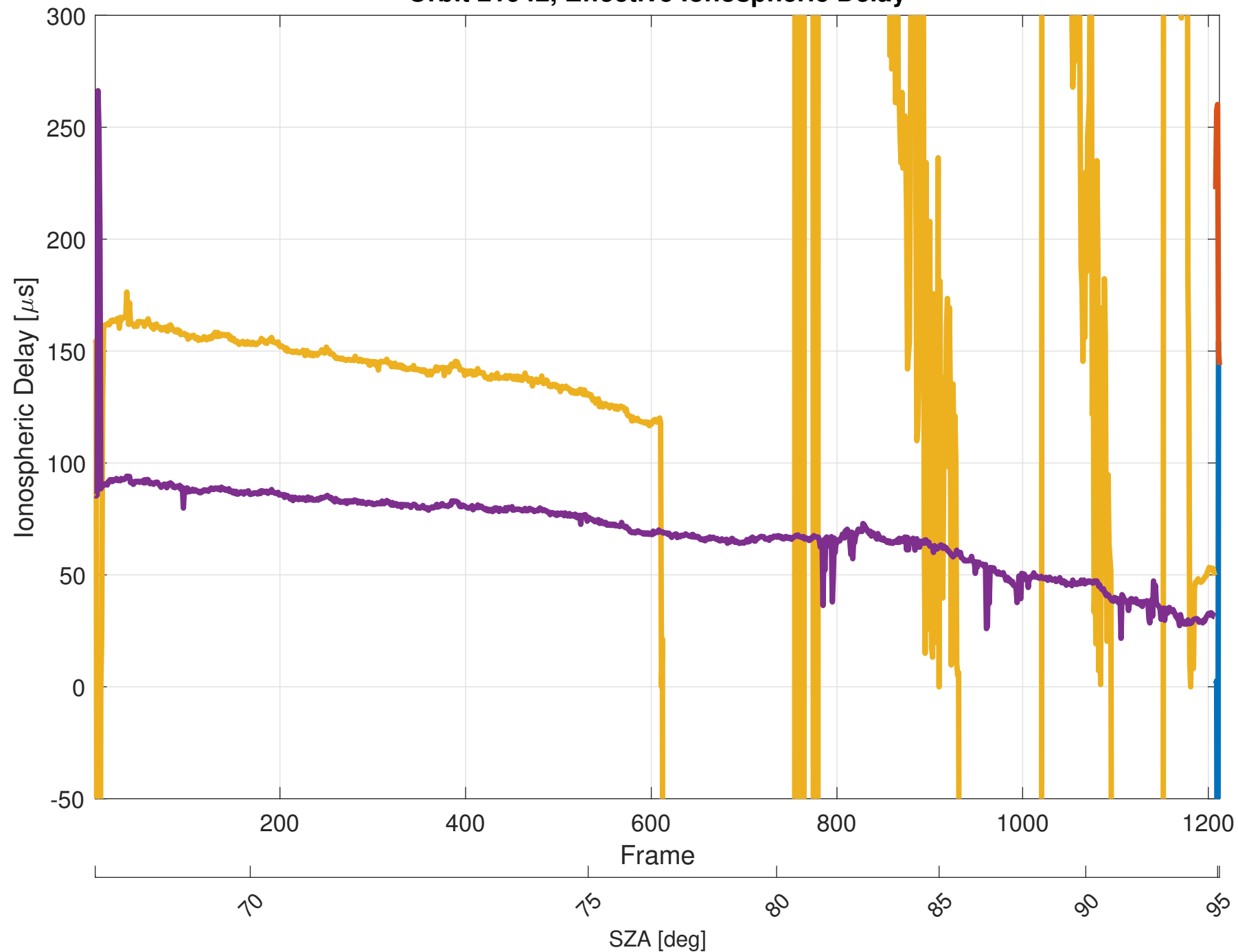
Orbit 21942, Effective Ionospheric Delay
