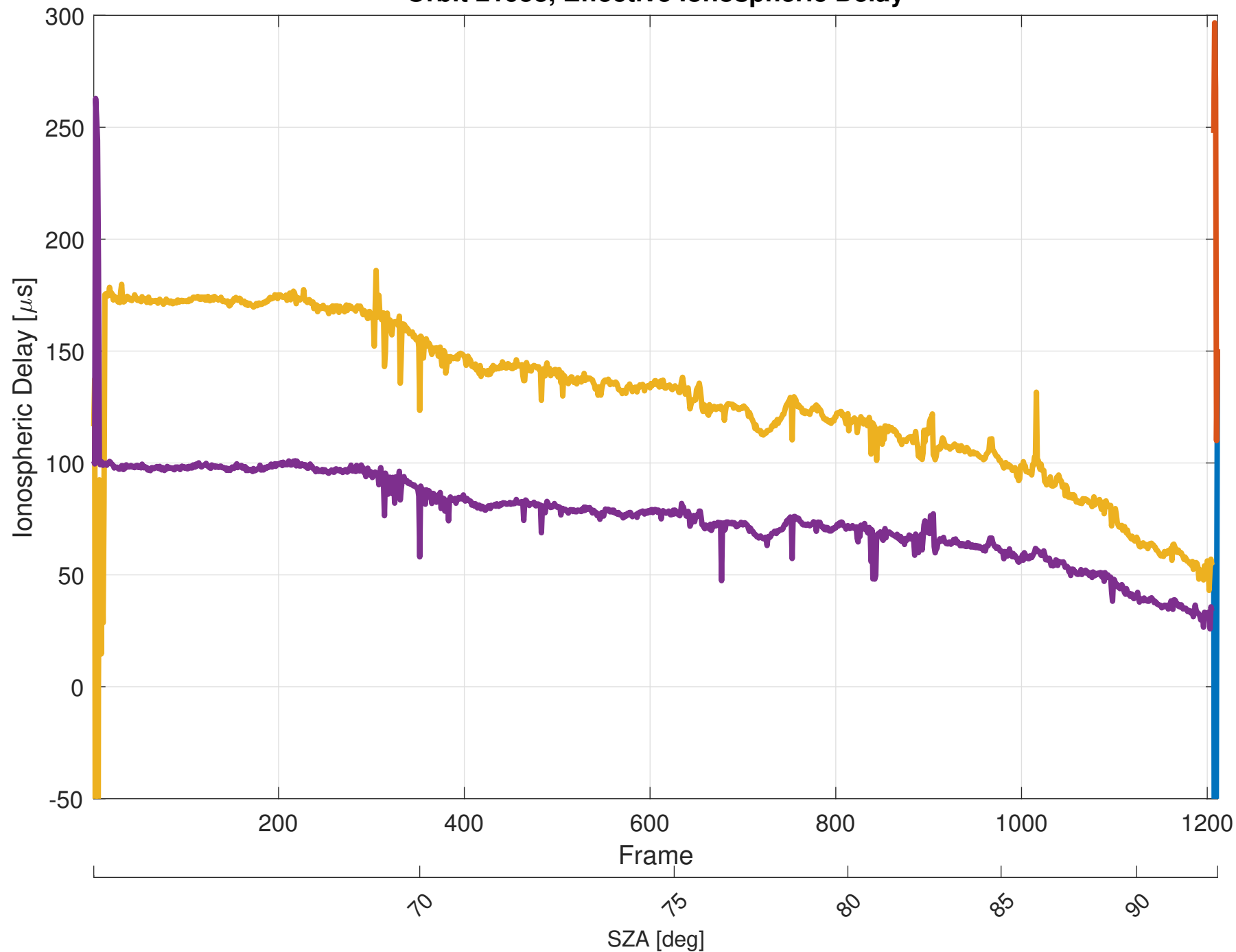
Orbit 21953, Effective Ionospheric Delay
