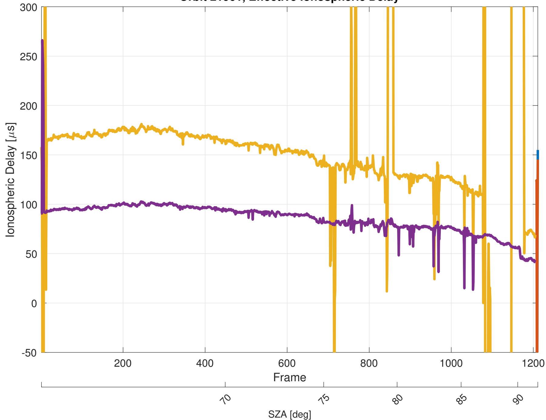
Orbit 21961, Effective Ionospheric Delay
