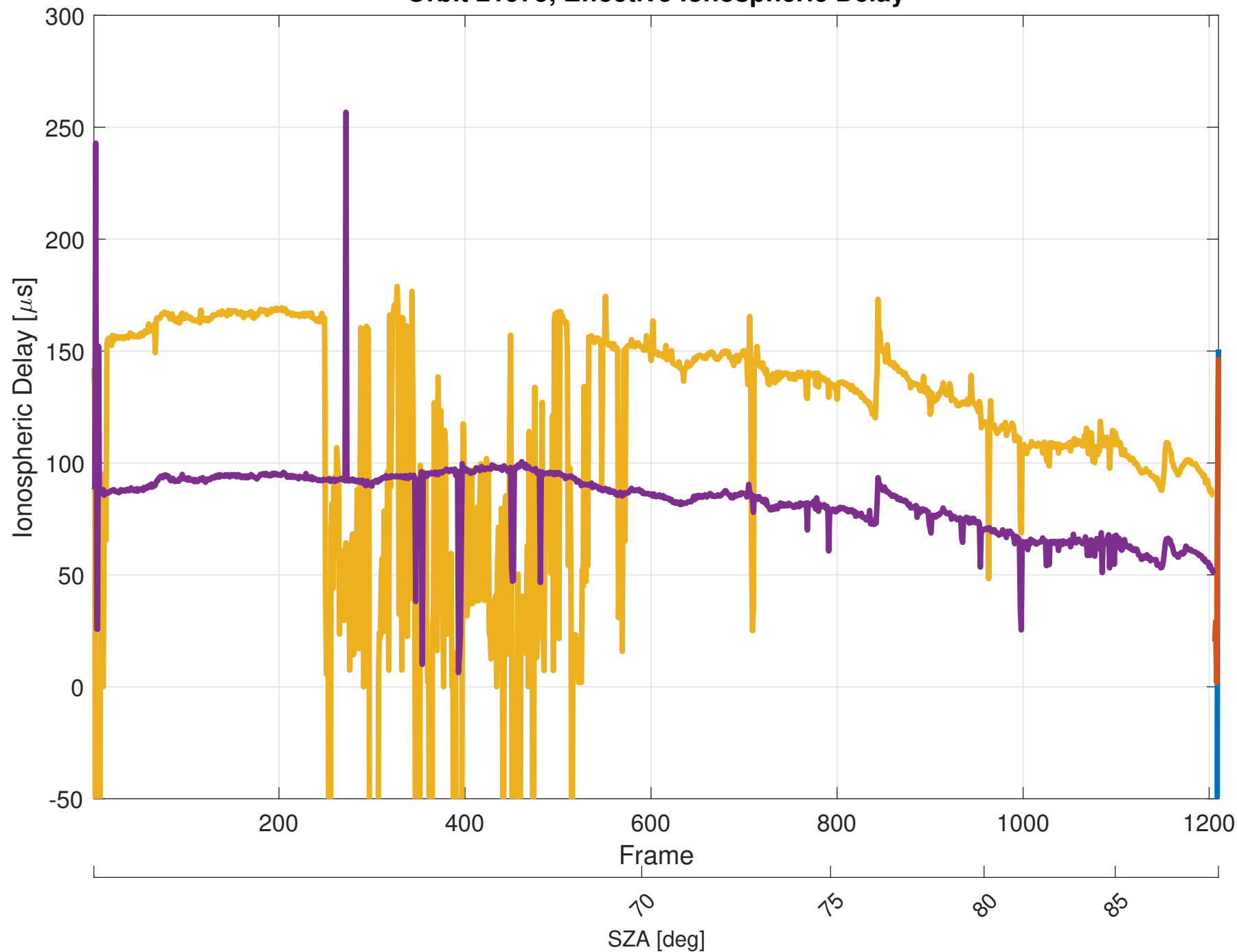
Orbit 21975, Effective Ionospheric Delay
