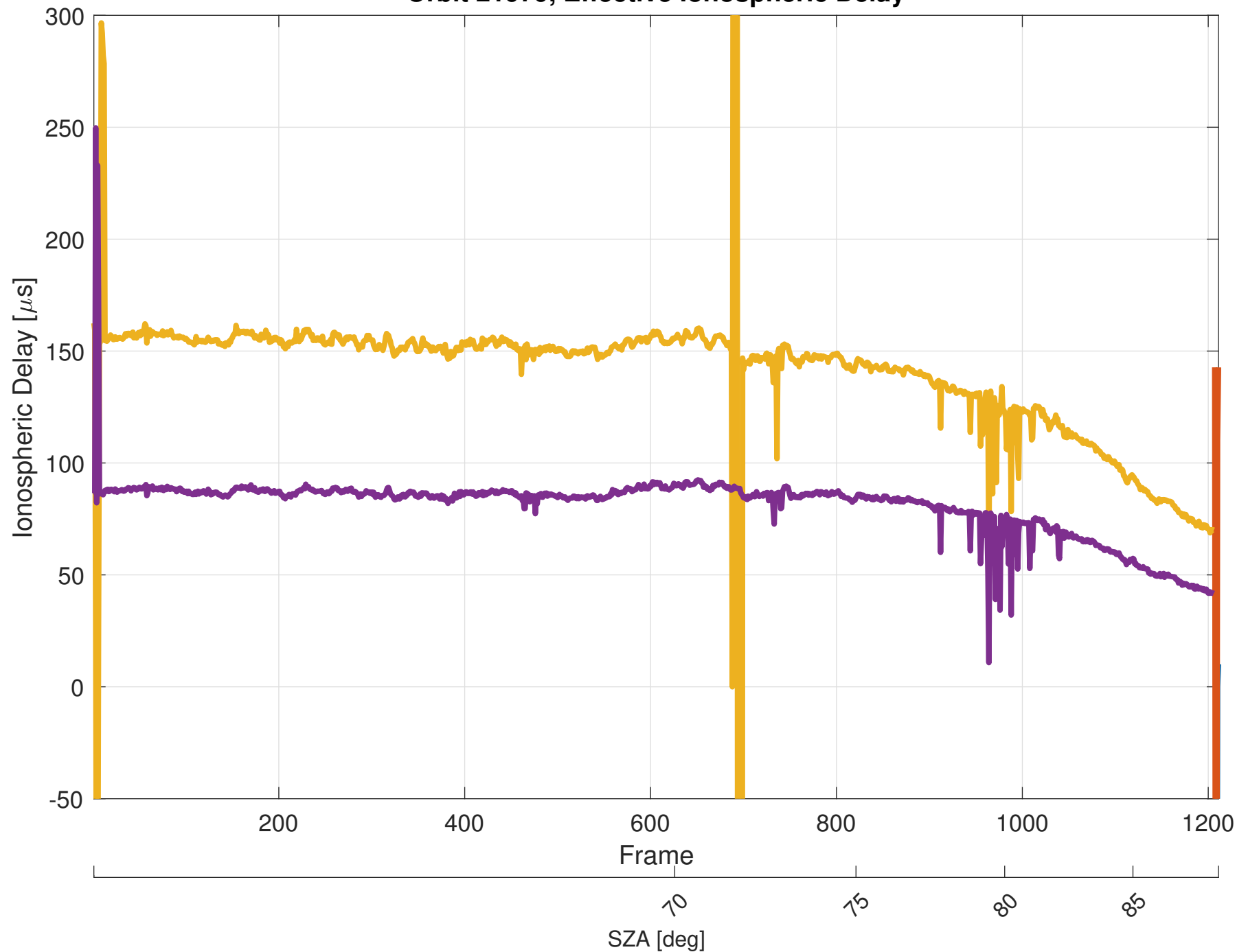
Orbit 21979, Effective Ionospheric Delay
