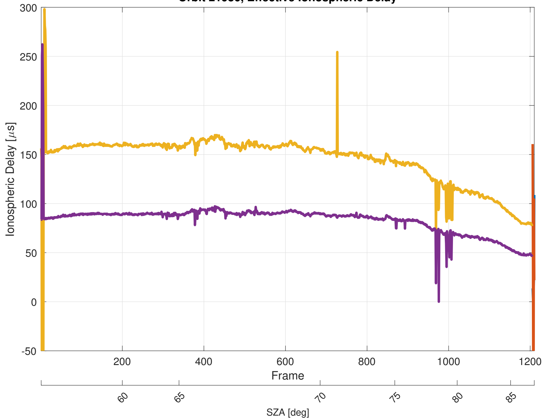
Orbit 21986, Effective Ionospheric Delay
