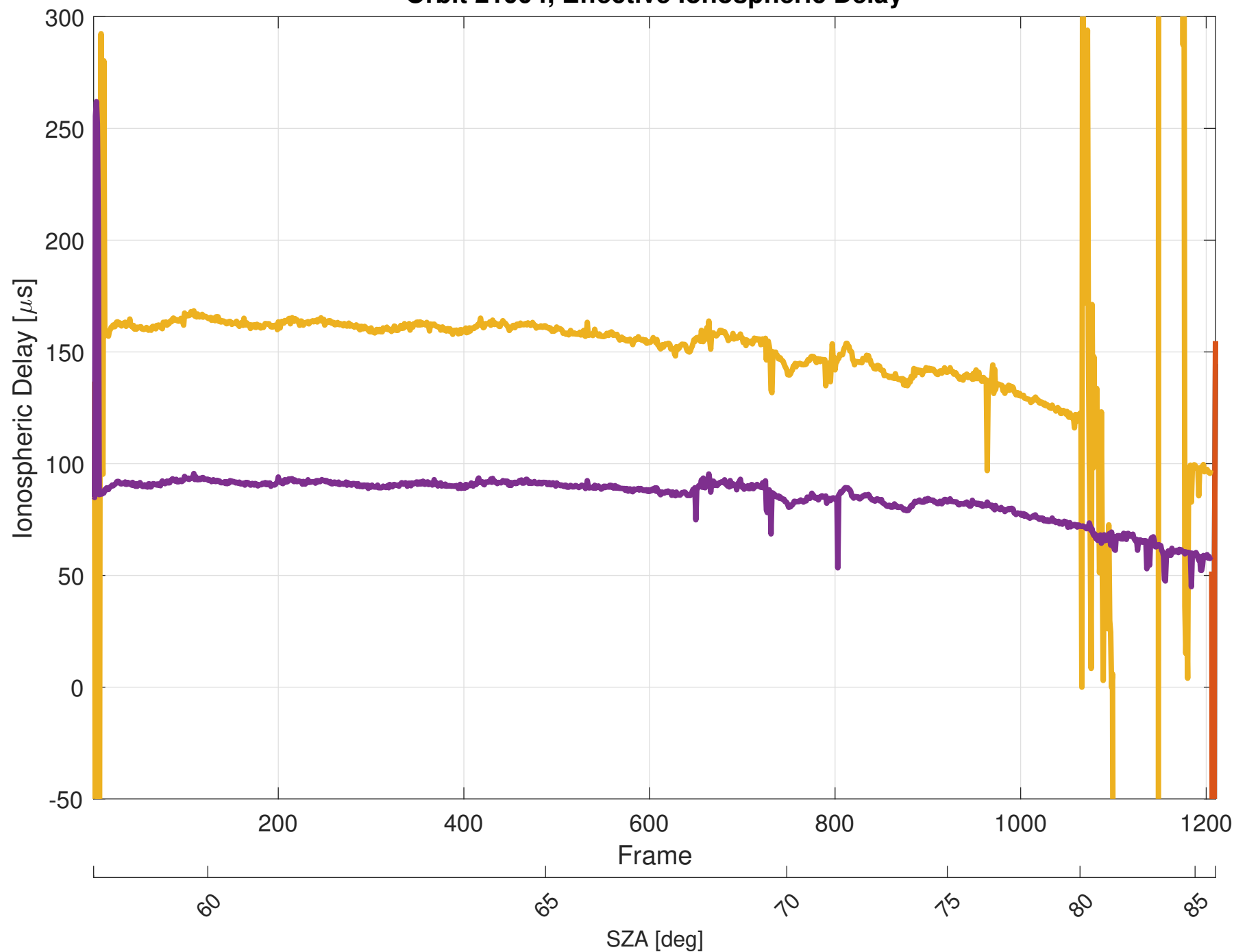
Orbit 21994, Effective Ionospheric Delay
