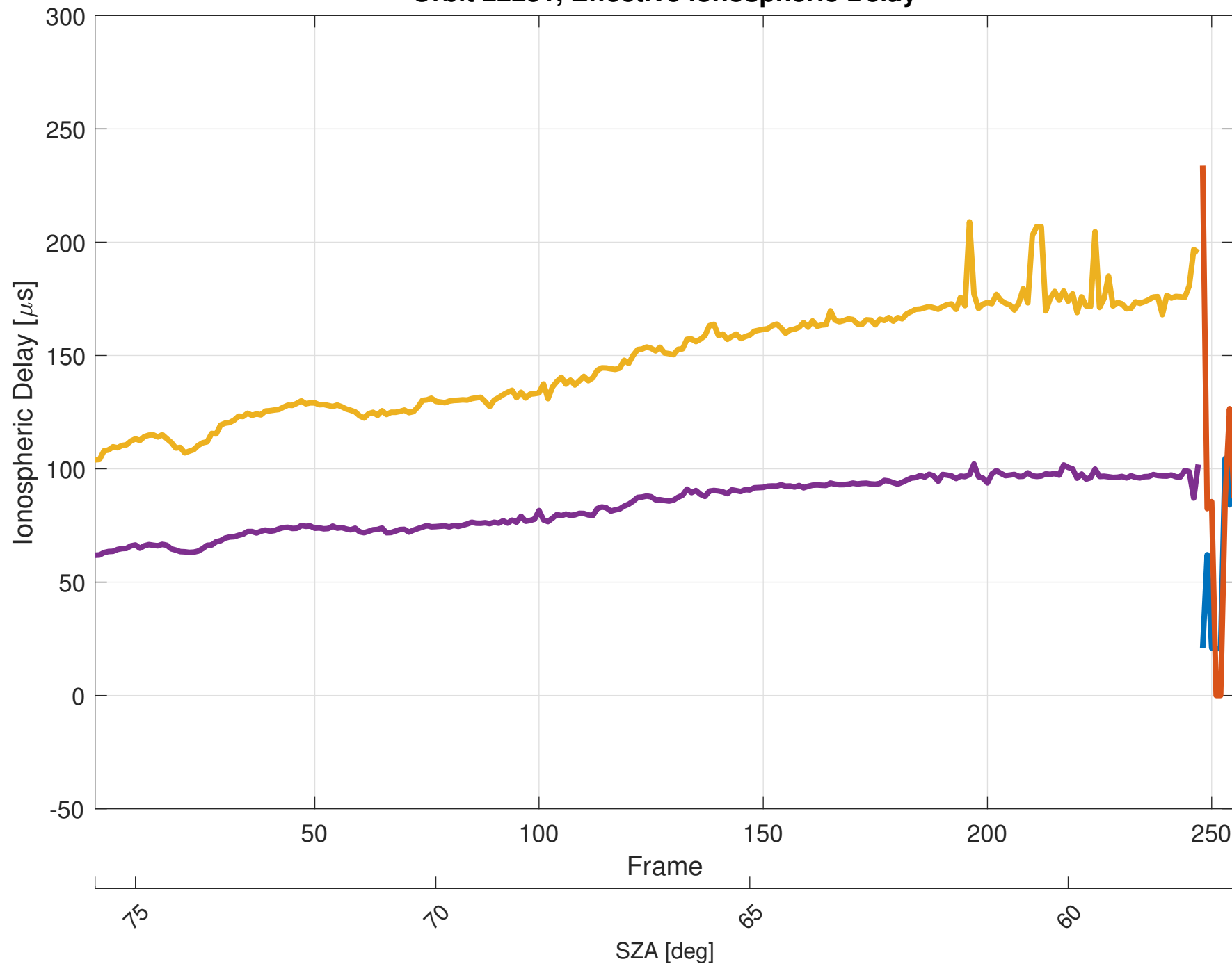
Orbit 22251, Effective Ionospheric Delay
